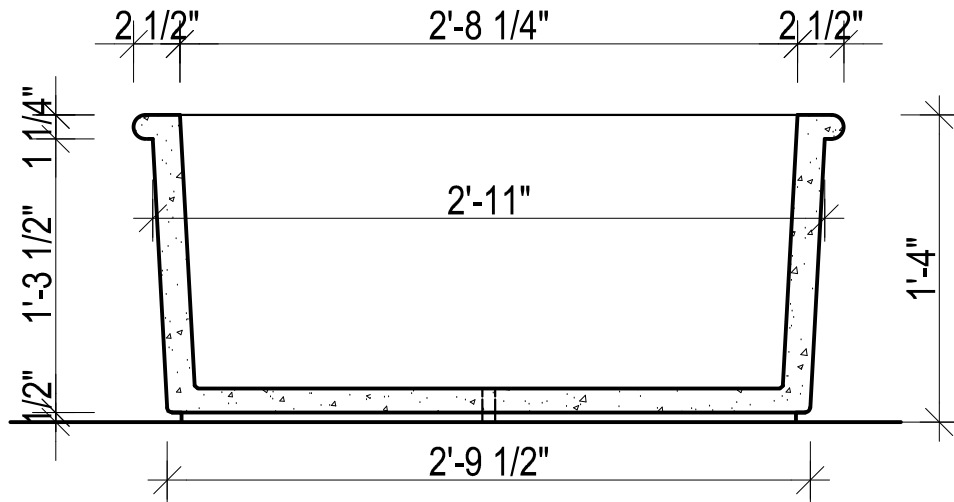
SECTION
