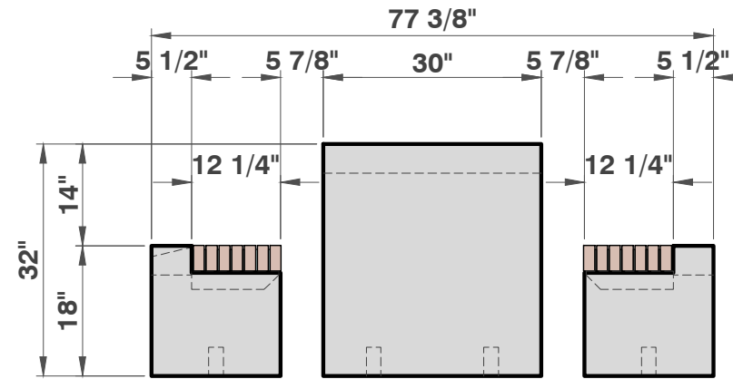
END VIEW 1/2" = 1'
