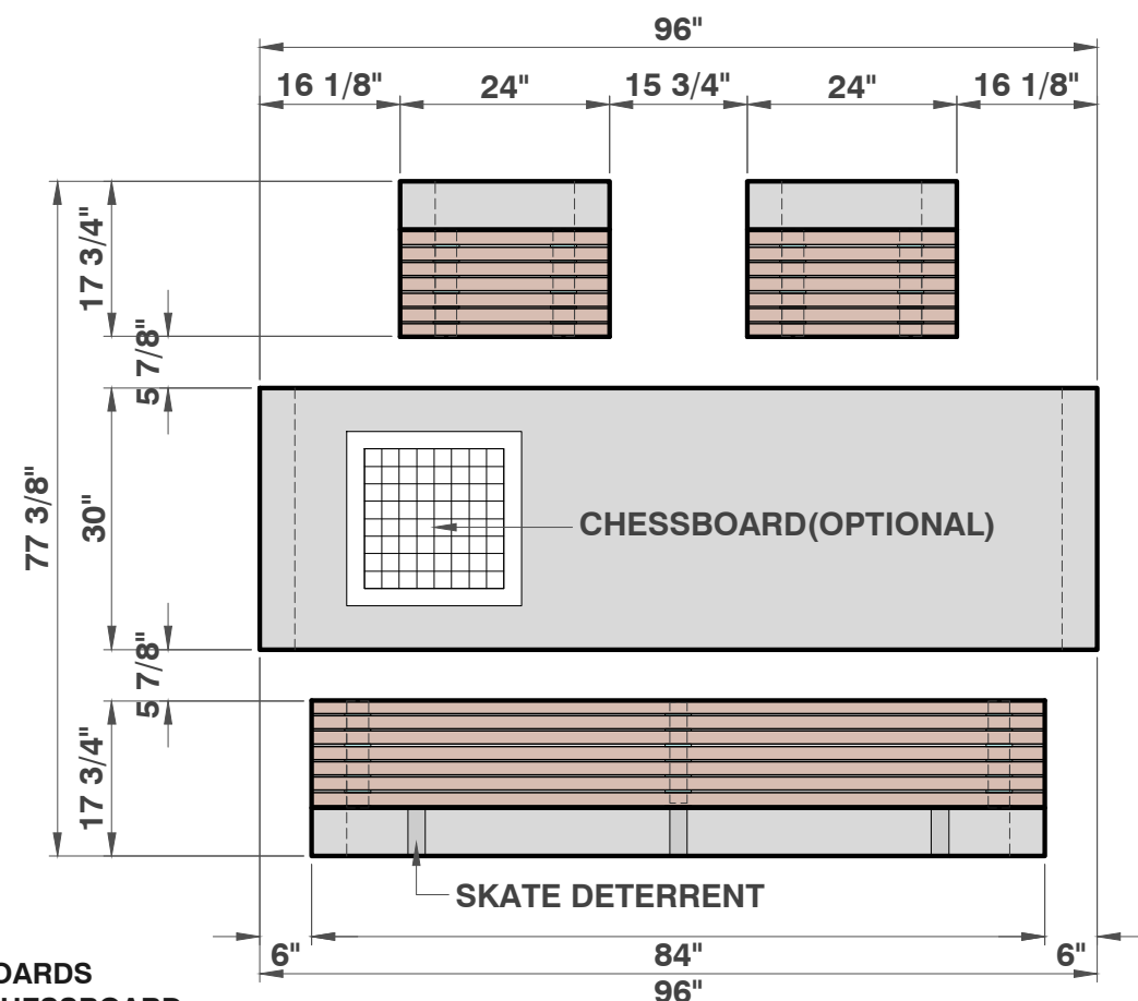
TOP VIEW 1/2" = 1'
