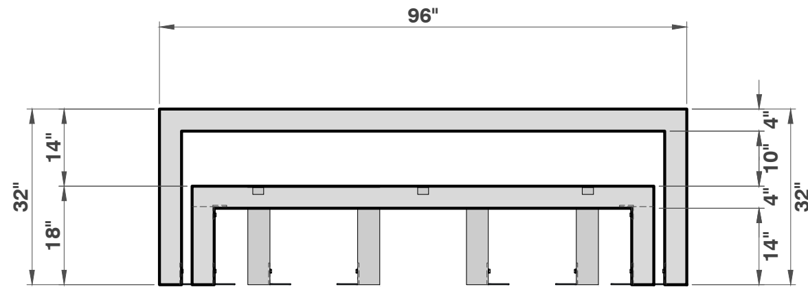
ELEVATION 1/2" = 1'
