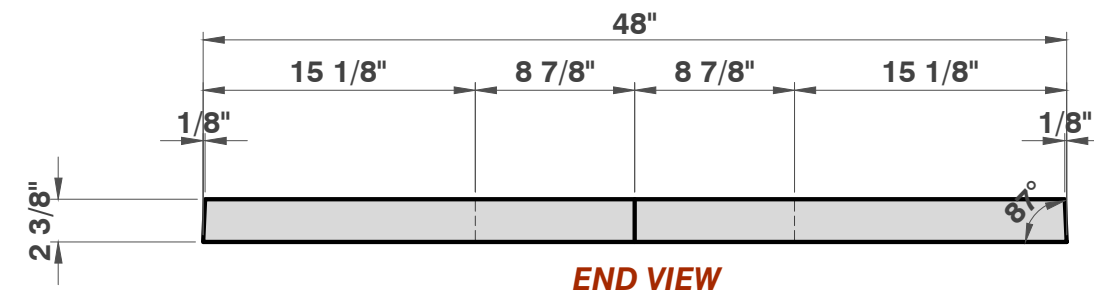
END VIEW 1 1/8" = 1'
