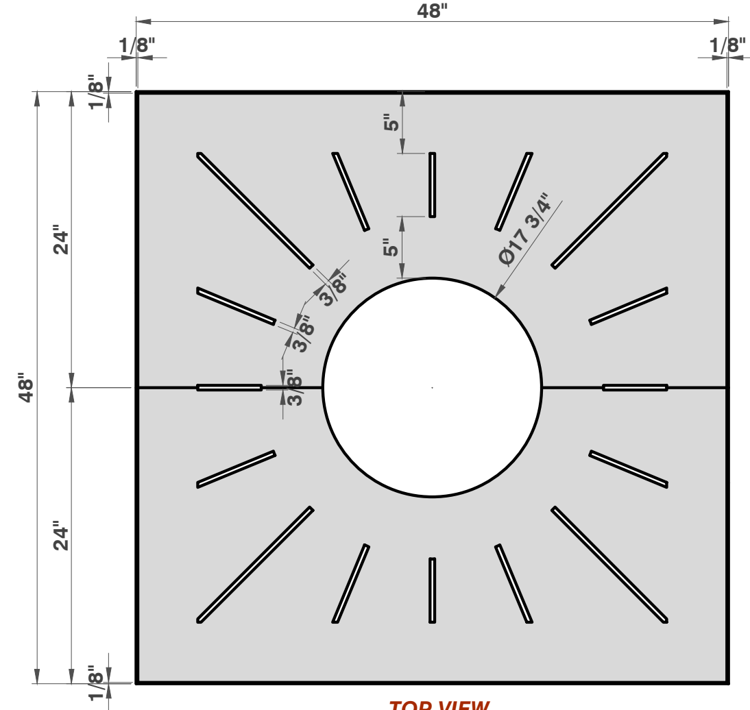
TOP VIEW 1 1/8" = 1'
