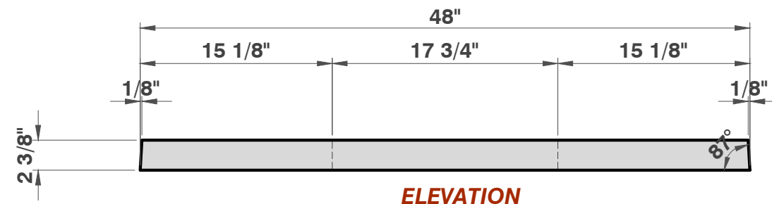
ELEVATION 1 1/8" = 1'
