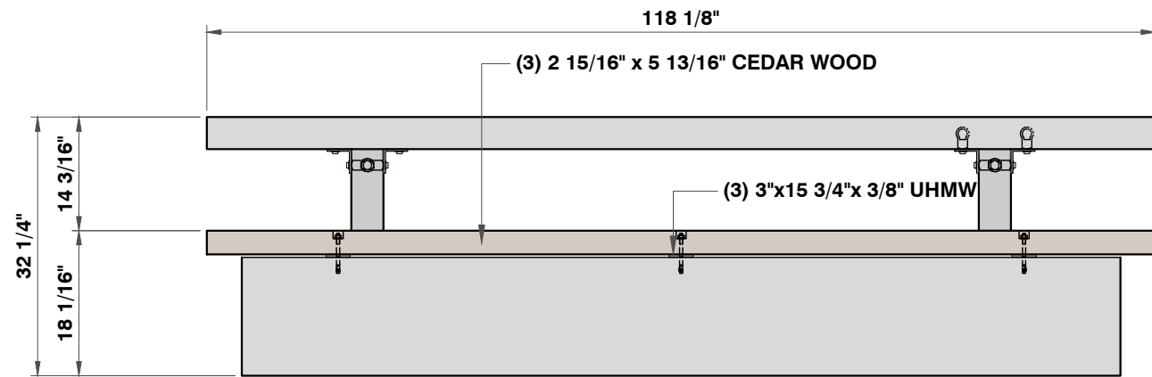
FRONT VIEW 9/16"=1'
