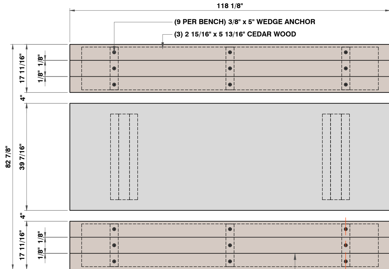
TOP VIEW 9/16"=1'
