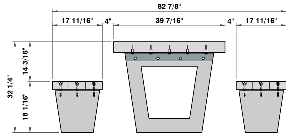
RIGHT SIDE VIEW 9/16"=1'
