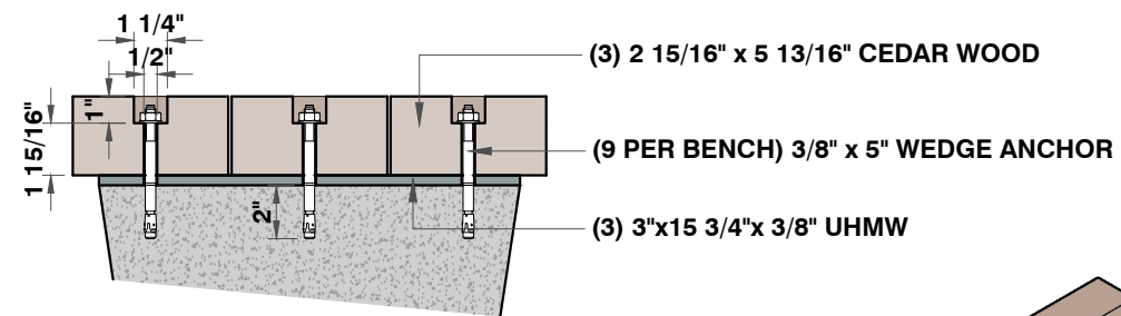
SECTION - A 1 1/2"=1'
