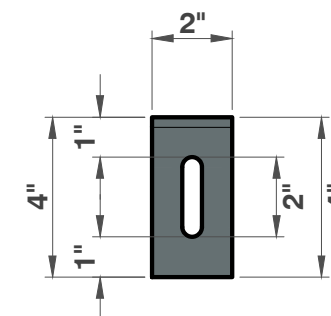
TOP VIEW 2 1/2"=1'
