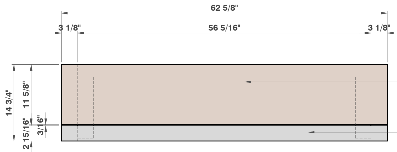
TOP VIEW 1 1/8" = 1'
