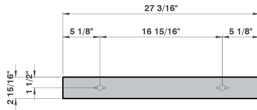
TOP VIEW 1 1/2" = 1'
