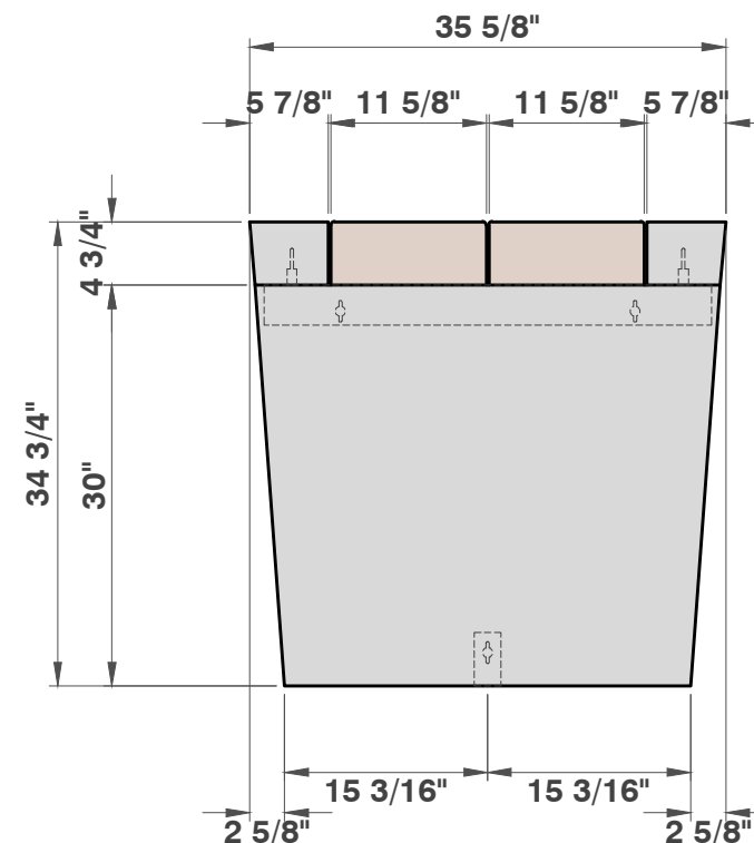
END VIEW 3/4" = 1'
