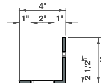
SECTION 2 1/2"=1'
