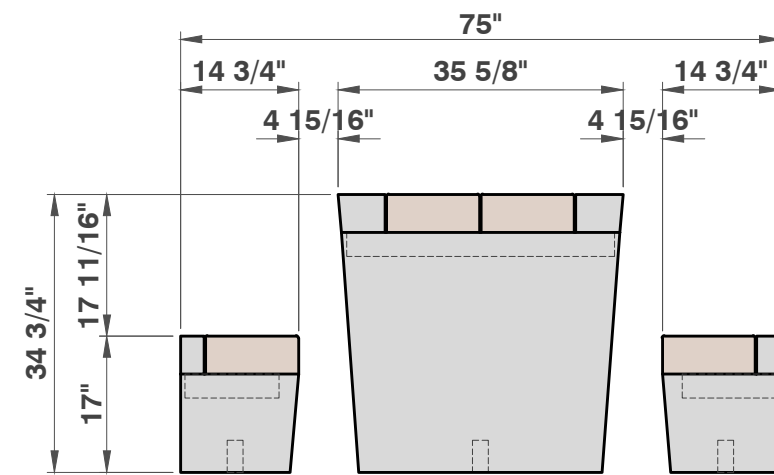
END VIEW 1/2" = 1'
