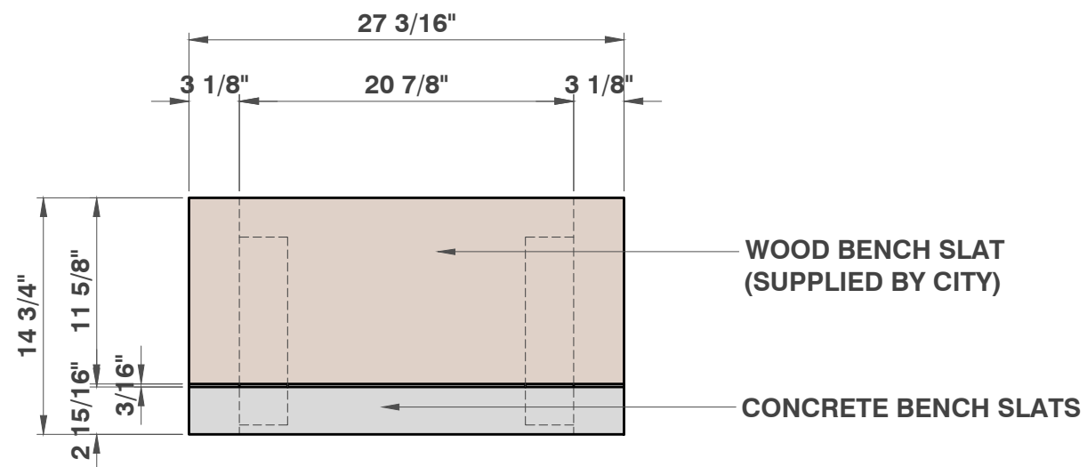
TOP VIEW 1 1/8" = 1'
