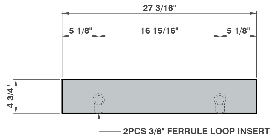
ELEVATION 1 1/2" = 1'
