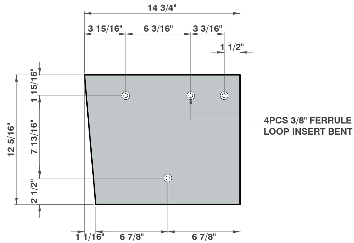
ELEVATION 2 1/8"=1'
