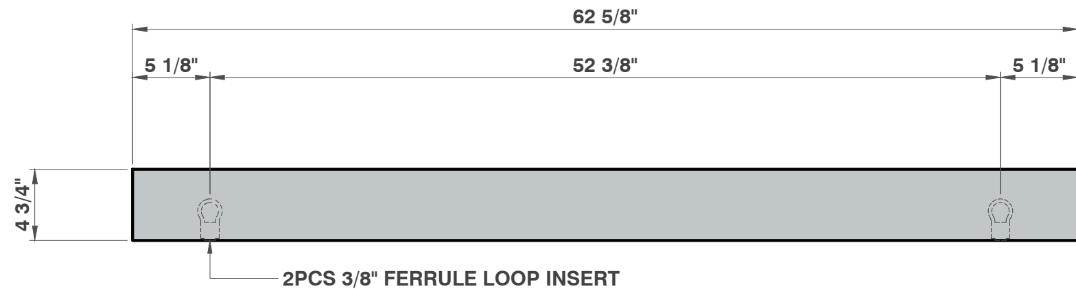
ELEVATION 1 3/8" = 1'
