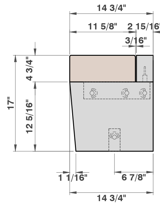
END VIEW 1 1/8" = 1'
