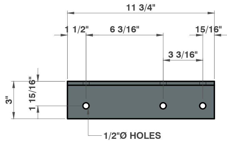
ELEVATION 2 1/2" = 1'
