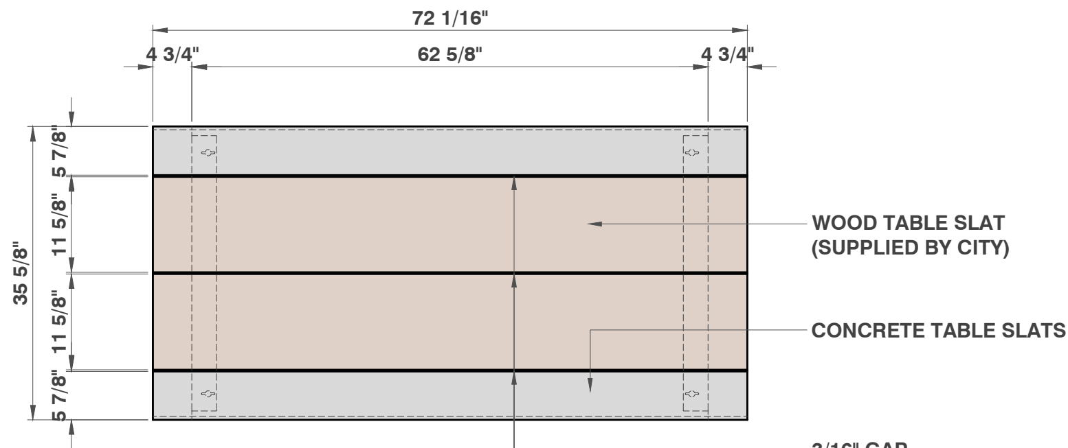
TOP VIEW 3/4" = 1'
