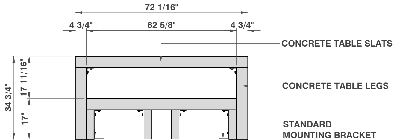
ELEVATION 1/2" = 1'
