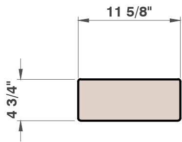
END VIEW 1 1/8"=1'
