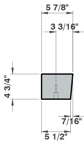
END VIEW 1 1/8" = 1'
