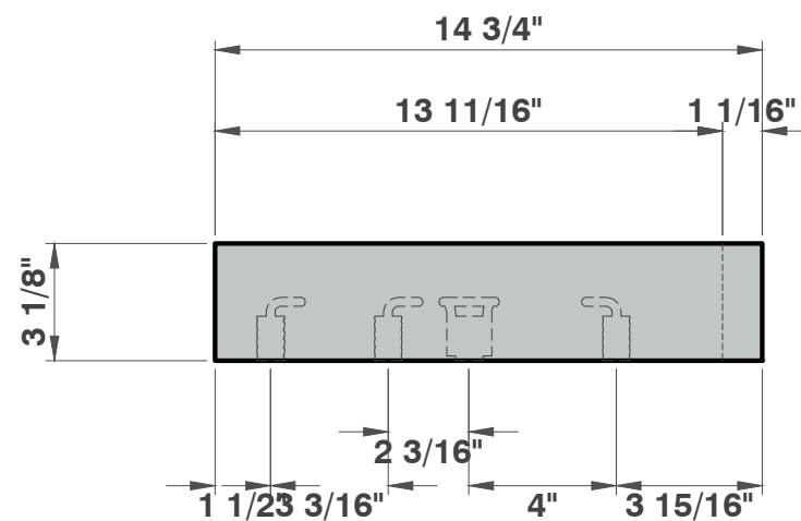
ELEVATION 2 1/8"=1'
