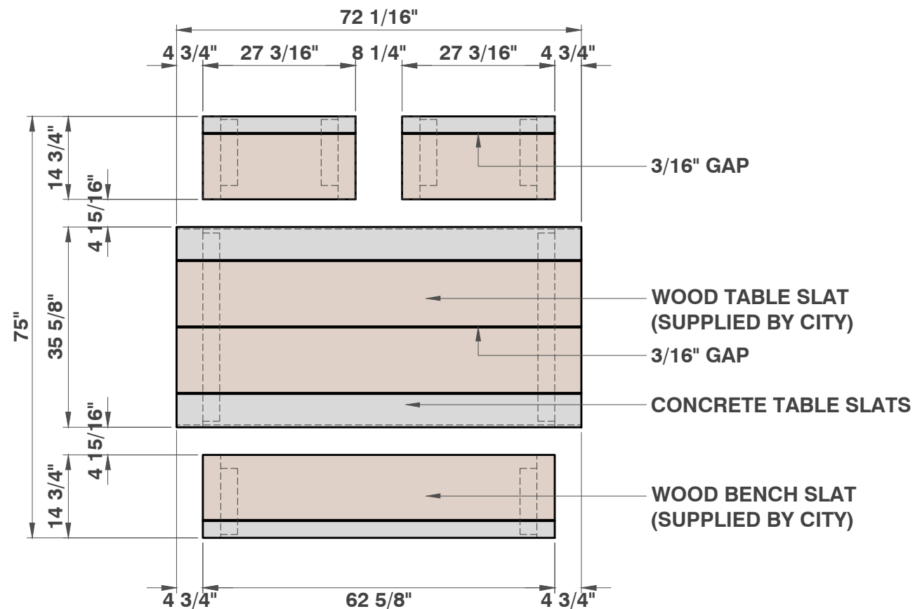
TOP VIEW 1/2" = 1'
