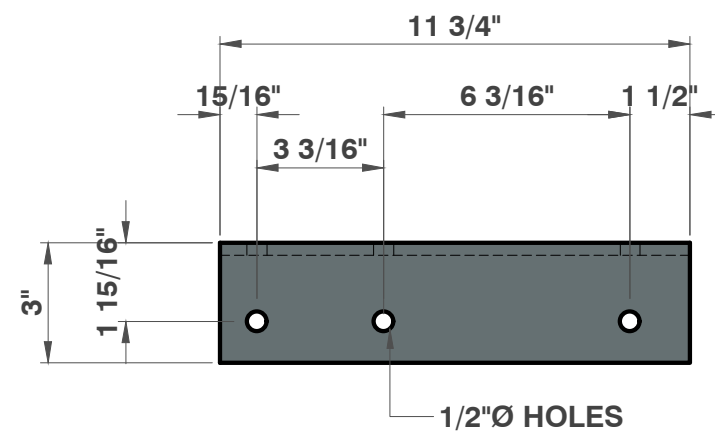
TOP VIEW 2 1/2" = 1'
