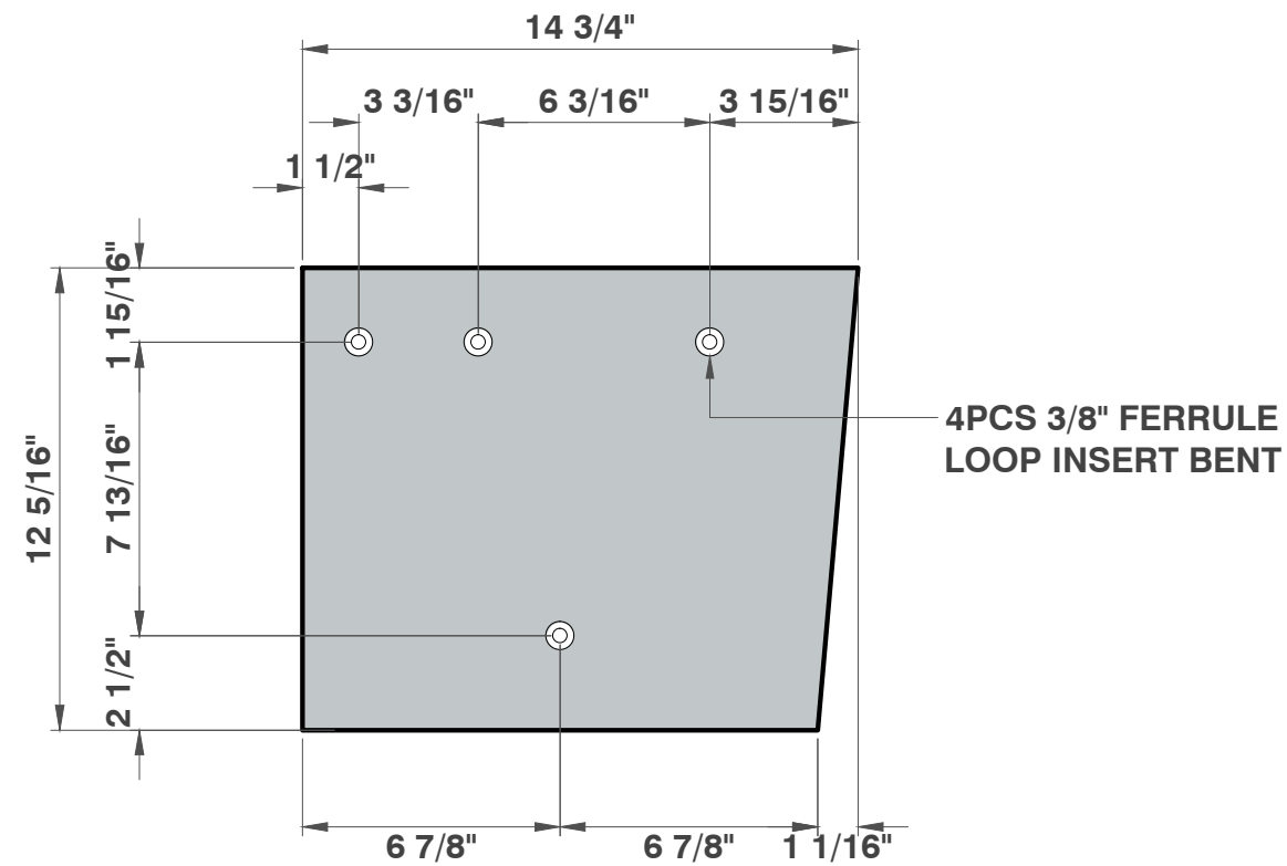
ELEVATION 2 1/8"=1'
