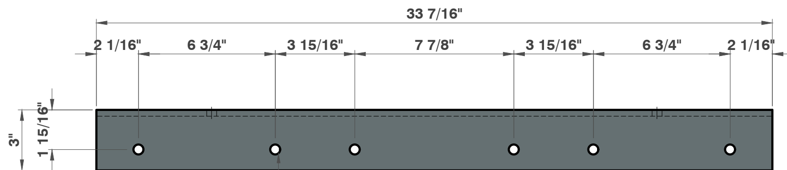
TOP VIEW 2 1/2"=1'
