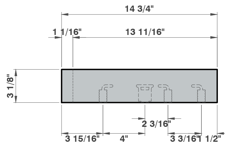
TOP VIEW 2 1/8"=1'
