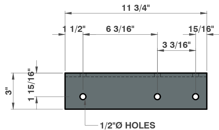
TOP VIEW 2 1/2" = 1'
