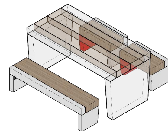
COMPLETE 3D PIECE ISOMETRIC VIEW
