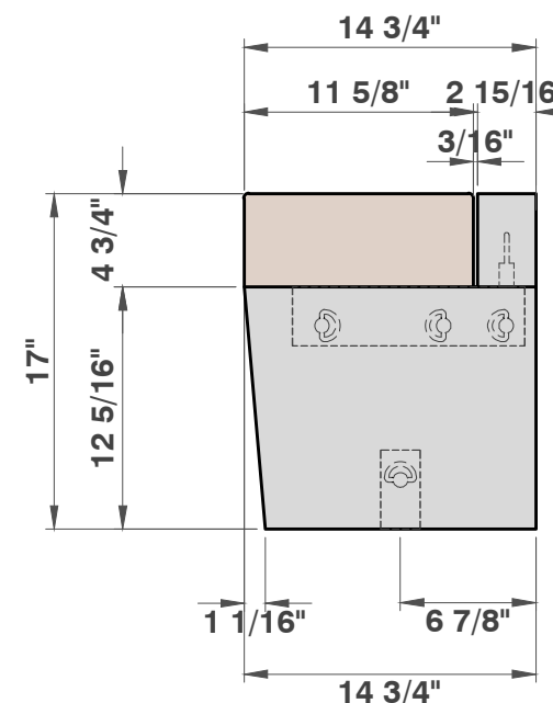
END VIEW 1 1/8" = 1'
