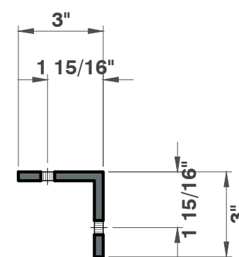
SECTION 2 1/2" = 1'
