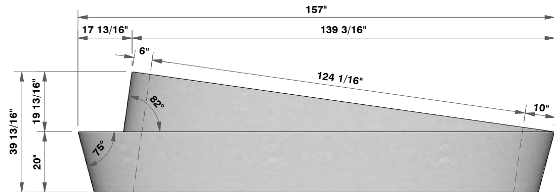
FRONT VIEW 3/8"=1'
