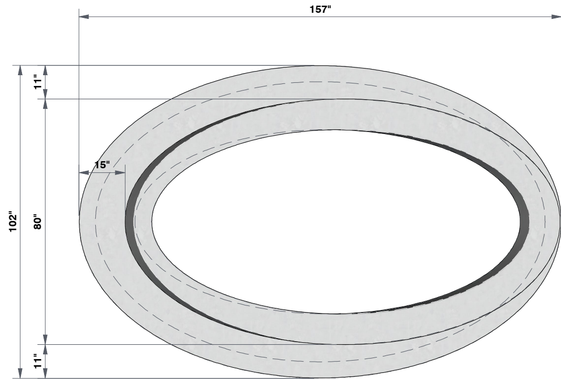
TOP VIEW 3/8"=1'
