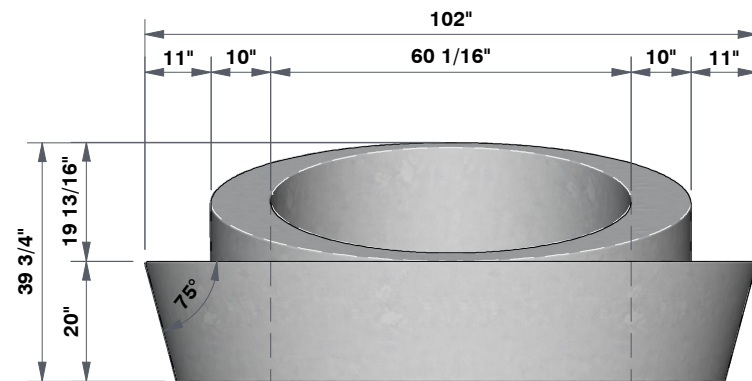
RIGHT SIDE VIEW 3/8"=1'
