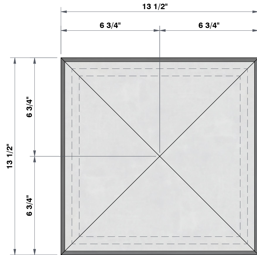
TOP VIEW 3"=1'
