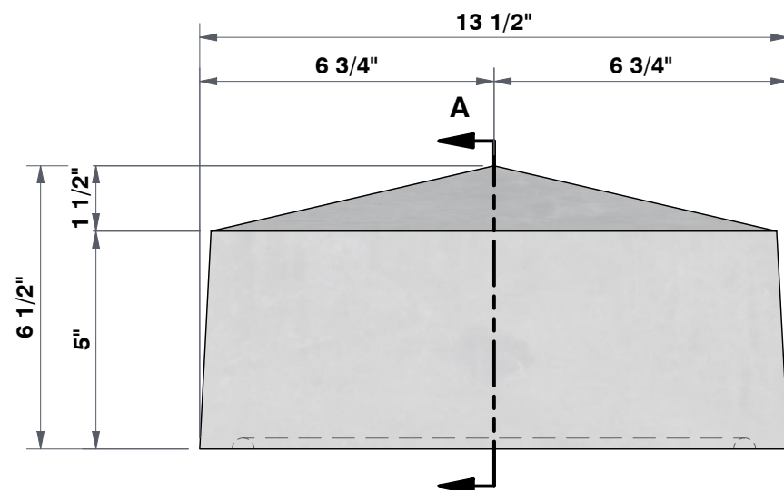
FRONT VIEW 3"=1'
