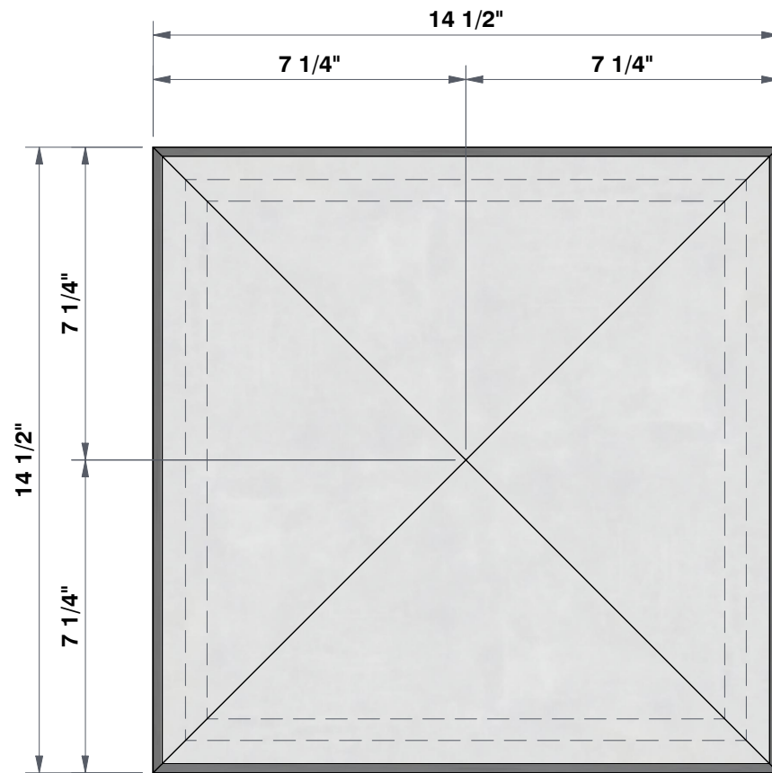
TOP VIEW 3"=1'
