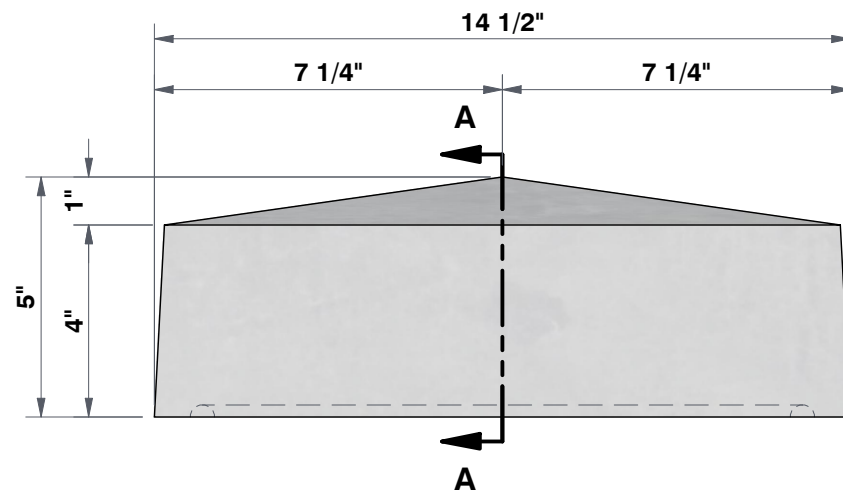
FRONT VIEW 3"=1'
