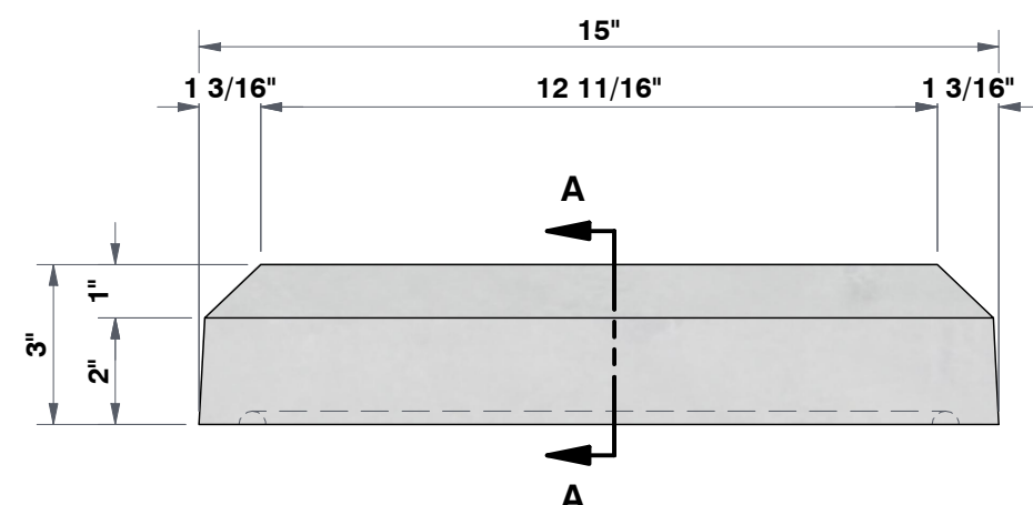
FRONT VIEW 3"=1'
