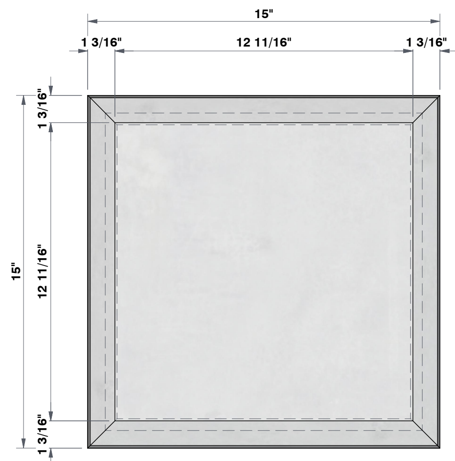
TOP VIEW 3"=1'
