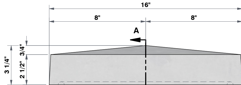
FRONT VIEW 3"=1'
