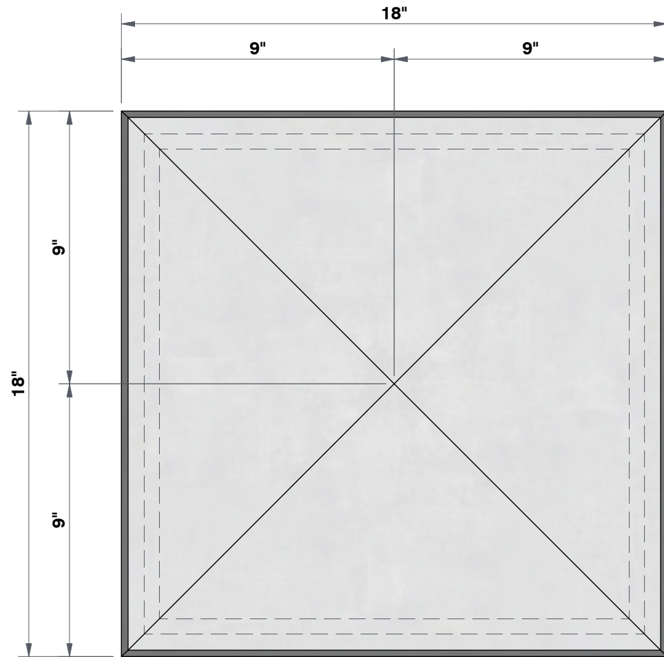
TOP VIEW 2 3/4"=1'
