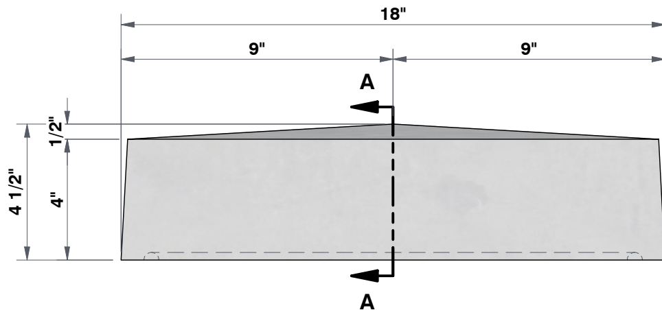
FRONT VIEW 2 3/4"=1'
