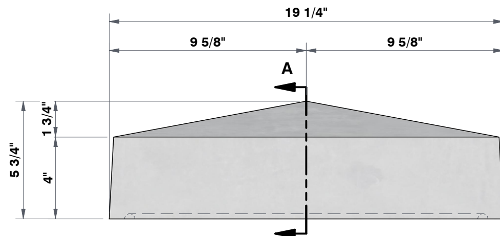
FRONT VIEW 2 1/2"=1'
