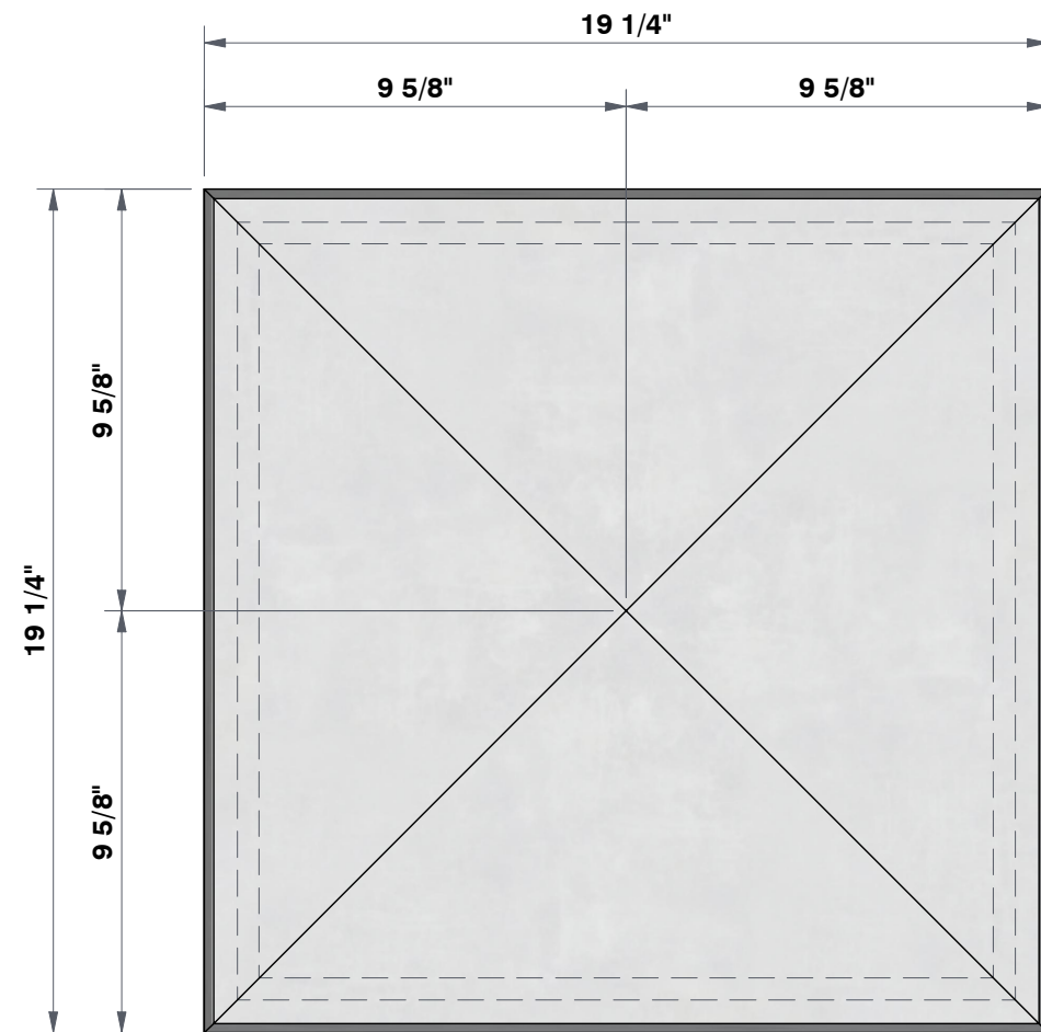
TOP VIEW 2 1/2"=1'
