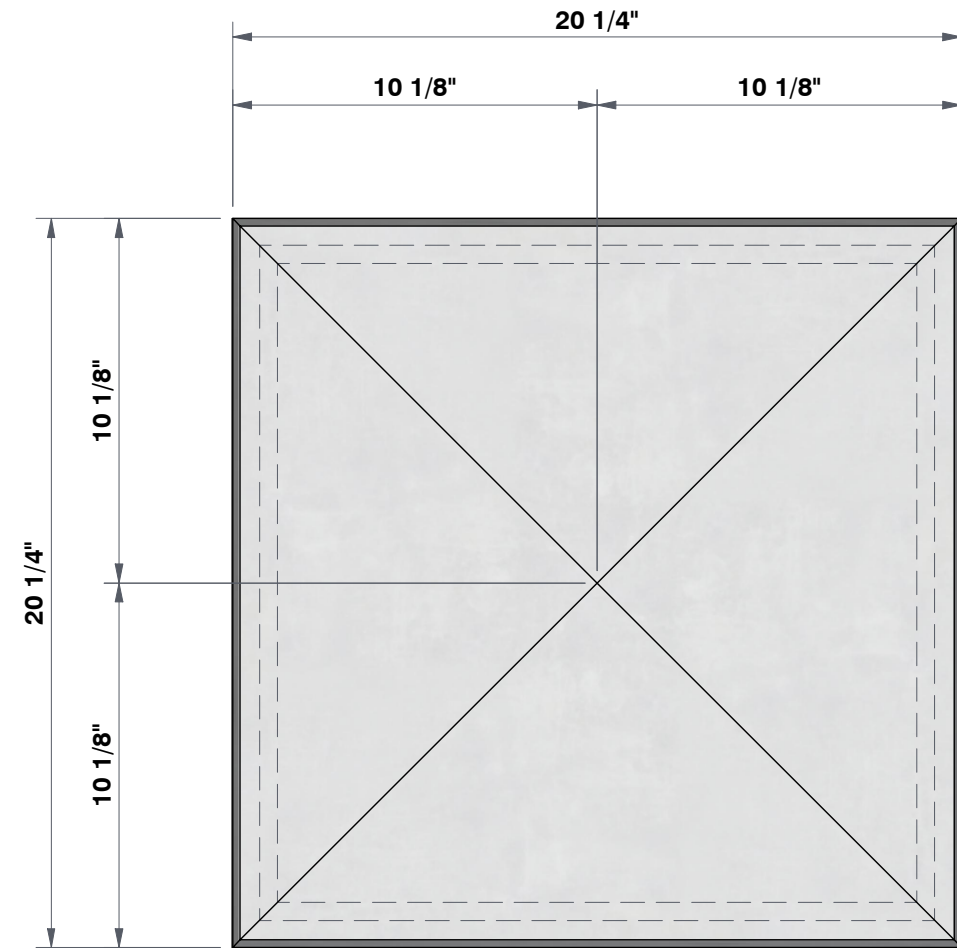
TOP VIEW 2 1/4"=1'
