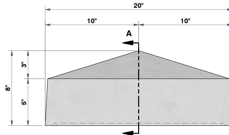
A FRONT VIEW 2 1/4"=1'
