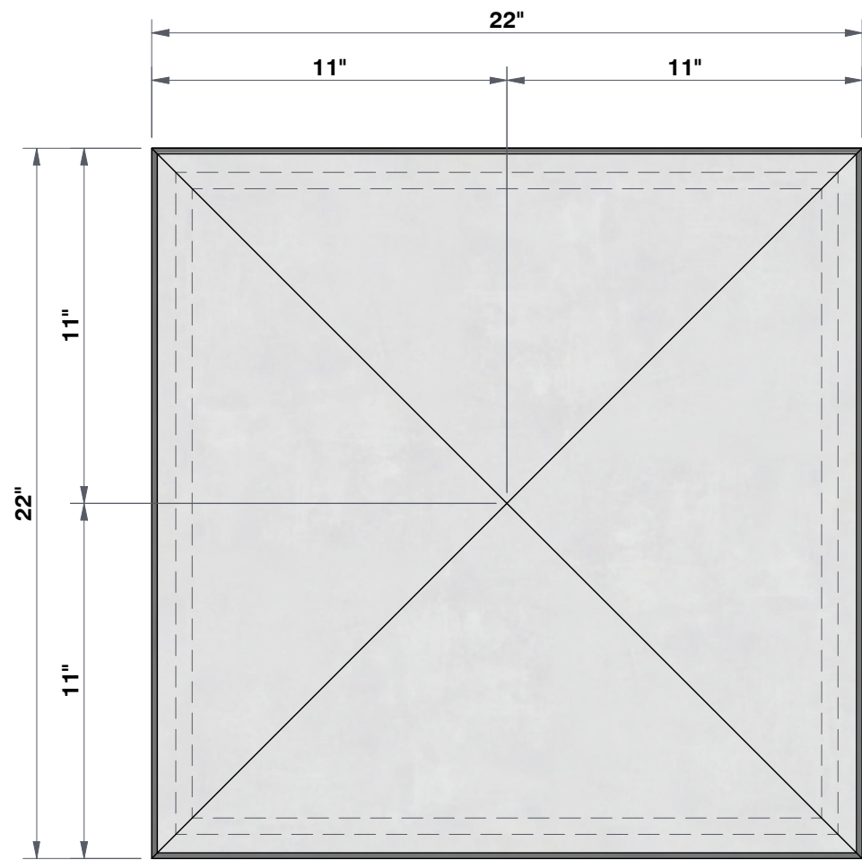
TOP VIEW 2 1/4"=1'
