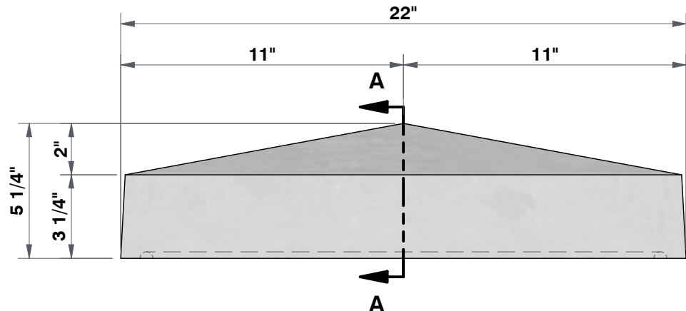
FRONT VIEW 2 1/4"=1'
