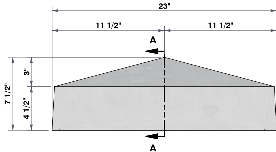
FRONT VIEW 2"=1'
