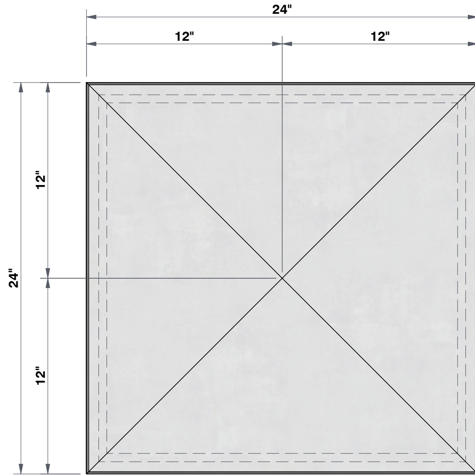
TOP VIEW 2"=1'
