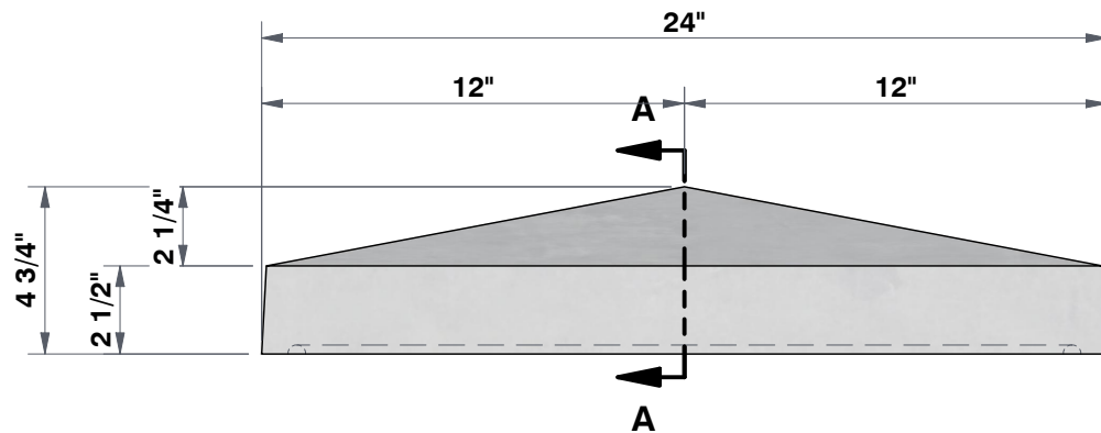
FRONT VIEW 2"=1'
