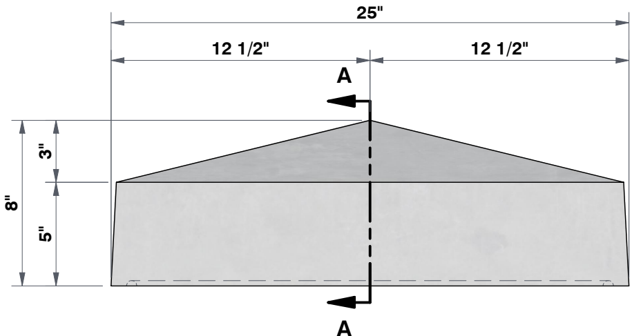
FRONT VIEW 1 7/8"=1'
