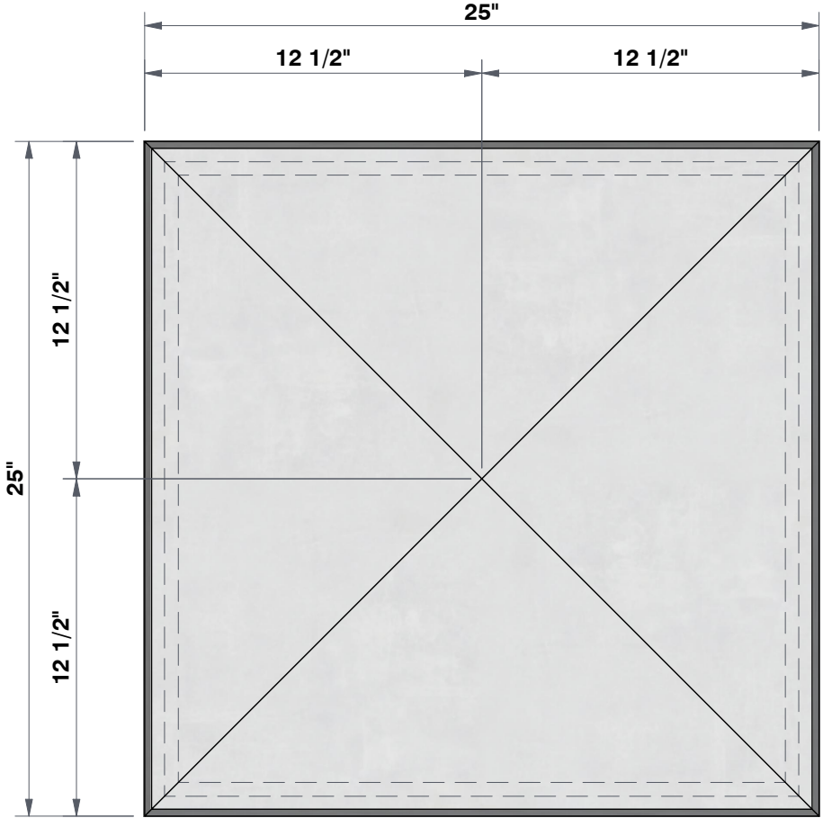
TOP VIEW 1 7/8"=1'
