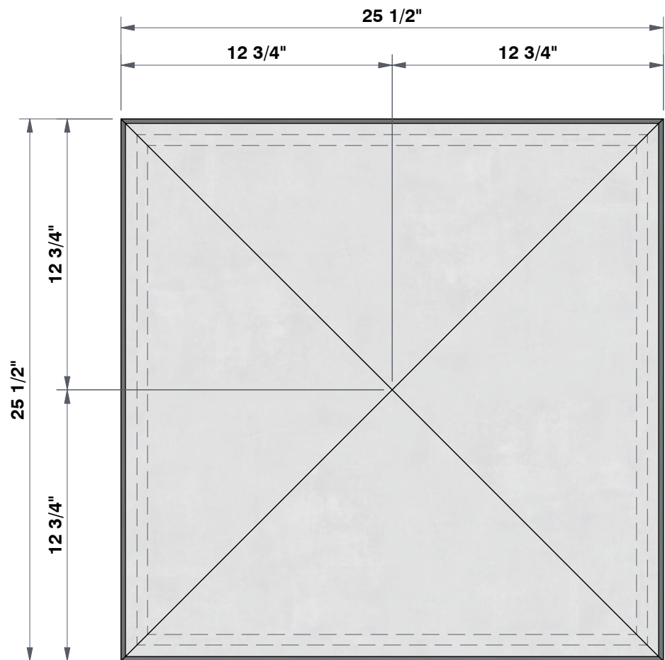
TOP VIEW 1 7/8"=1'
