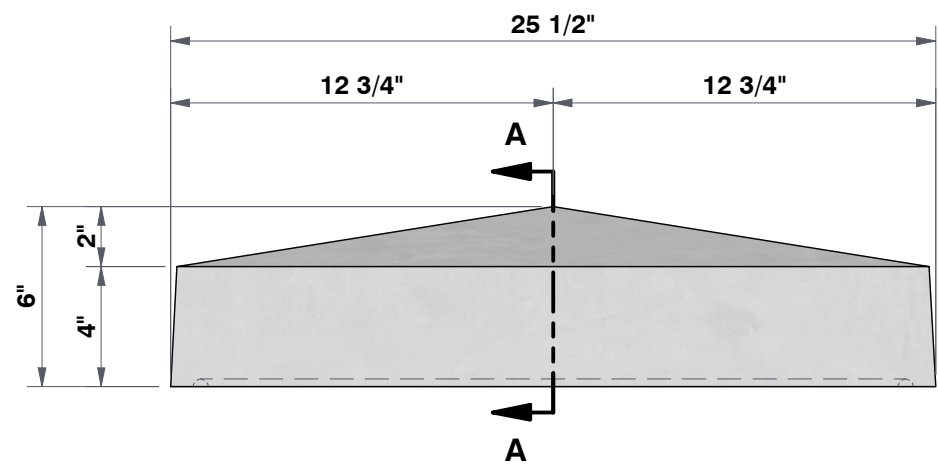
FRONT VIEW 1 7/8"=1'
