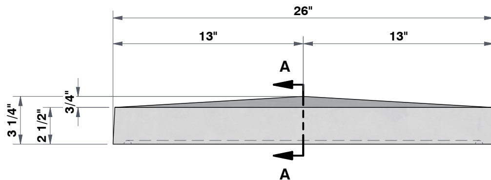
FRONT VIEW 1 7/8"=1'
