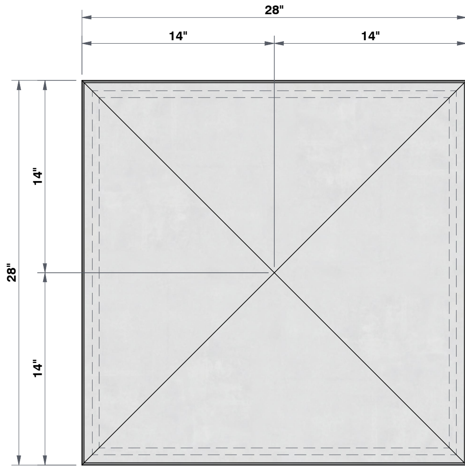
TOP VIEW 1 3/4"=1'
