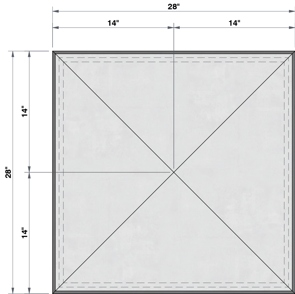
TOP VIEW 1 3/4"=1'
