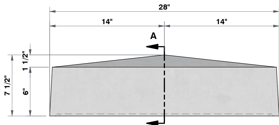
FRONT VIEW 1 3/4"=1'
