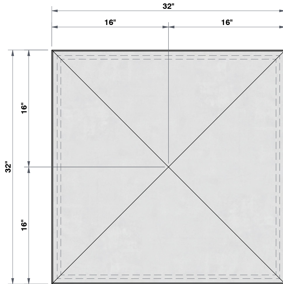
TOP VIEW 1 1/2"=1'
