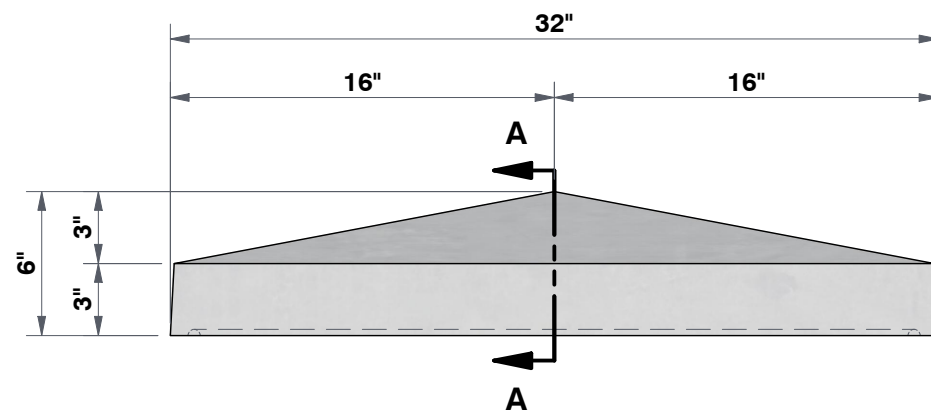
FRONT VIEW 1 1/2"=1'
