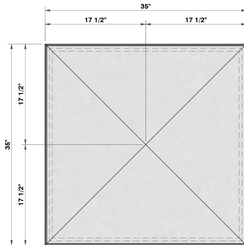
TOP VIEW 1 3/8"=1'
