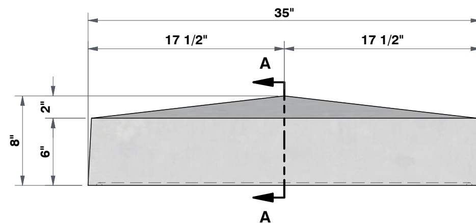
FRONT VIEW 1 3/8"=1'
