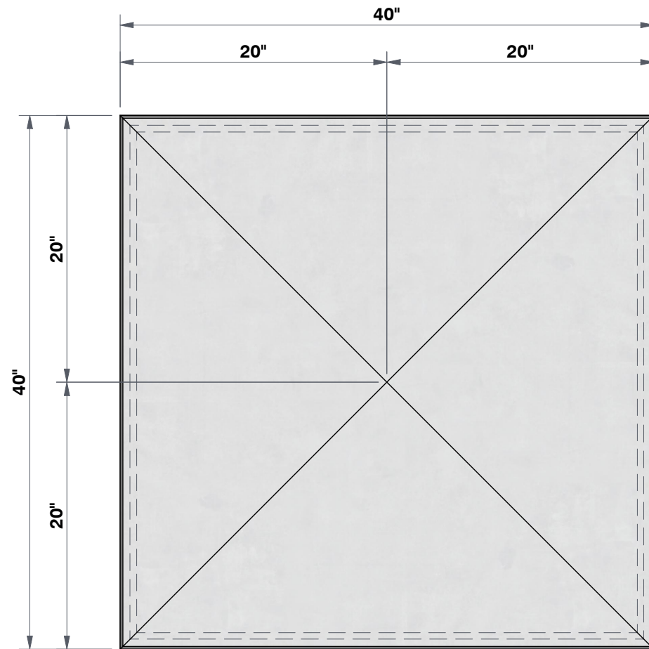
TOP VIEW 1 3/16"=1'
