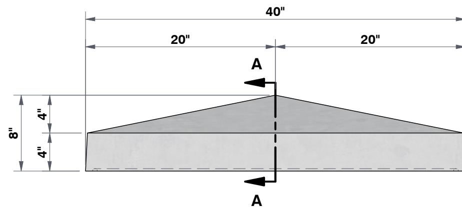
FRONT VIEW 1 3/16"=1'
