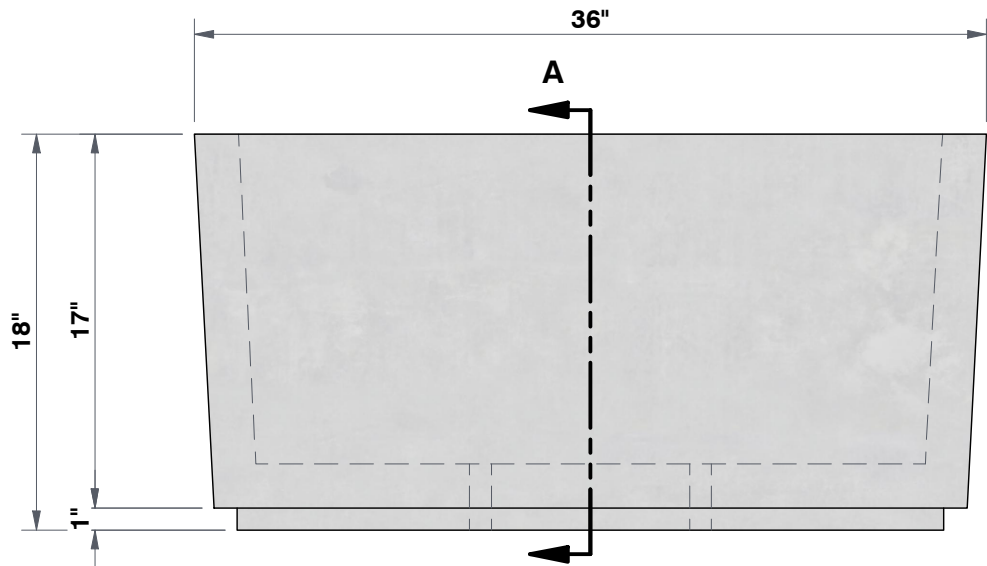
FRONT VIEW 1 3/8"=1'
