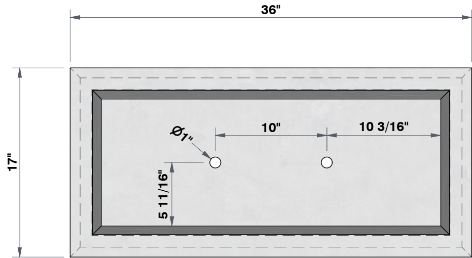
TOP VIEW 1 3/8"=1'
