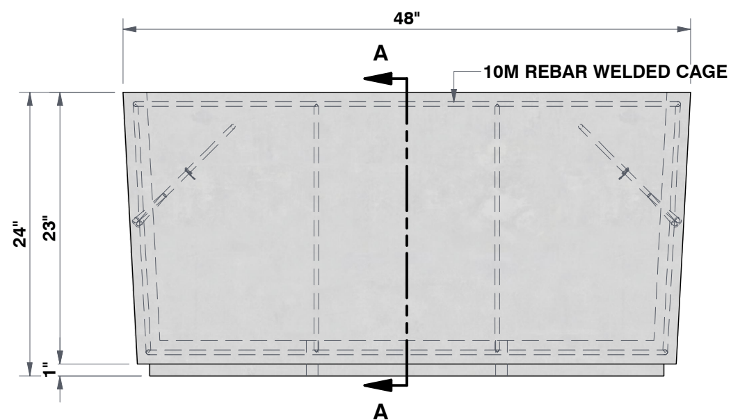
FRONT VIEW 1 1/16"=1'
