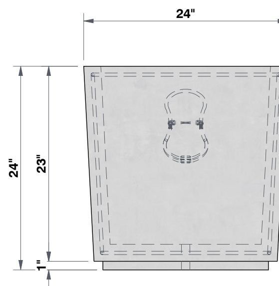
RIGHT SIDE VIEW 1 1/16"=1'
