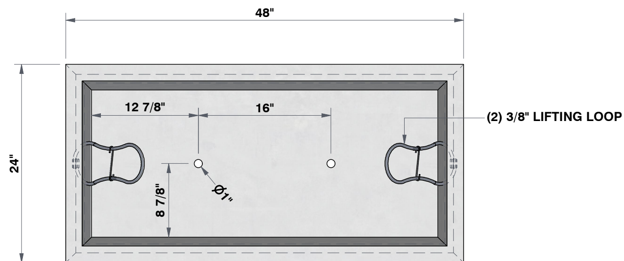
TOP VIEW 1 1/16"=1'
