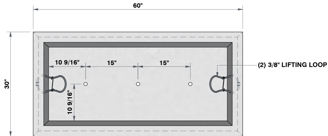
TOP VIEW 7/8"=1'
