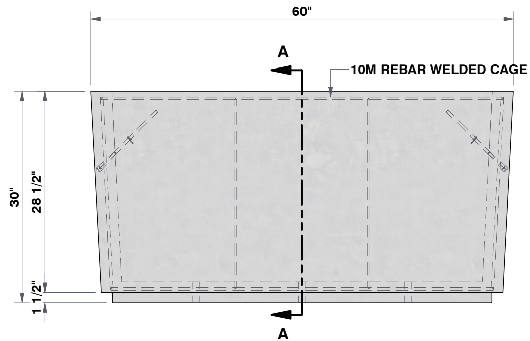
FRONT VIEW 7/8"=1'
