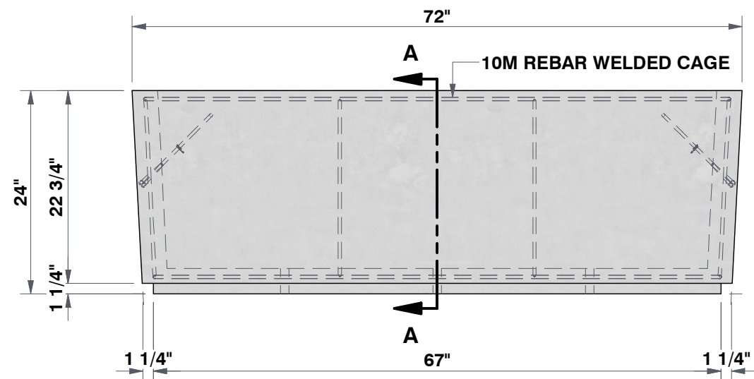
FRONT VIEW 3/4"=1'
