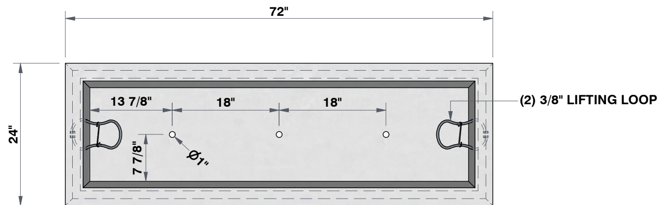
TOP VIEW 3/4"=1'
