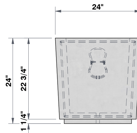
RIGHT SIDE VIEW 3/4"=1'
