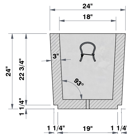
SECTION A-A 3/4"=1'
