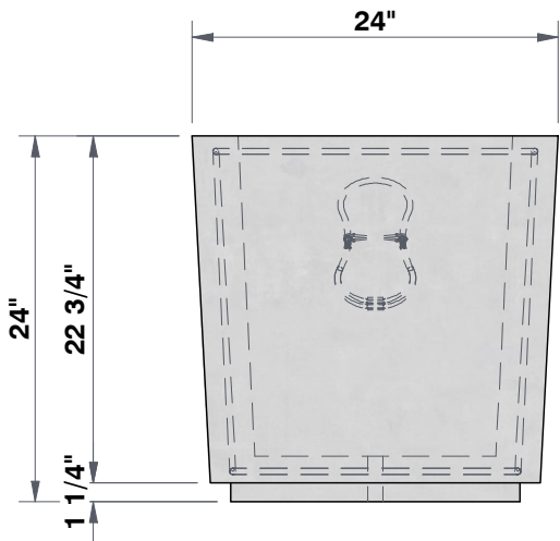
RIGHT SIDE VIEW 7/8"=1'
