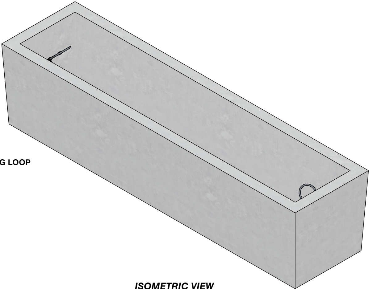
ISOMETRIC VIEW 7/8"=1'
