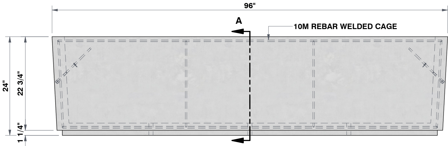
FRONT VIEW 7/8"=1'
