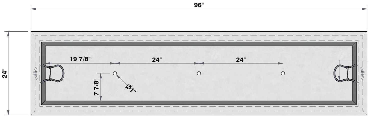
TOP VIEW 7/8"=1'
