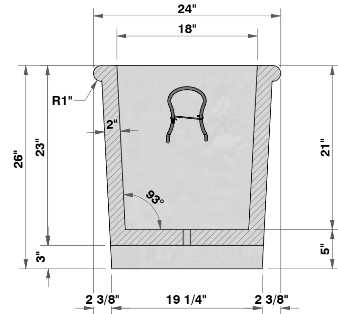
SECTION A-A 1"=1'
