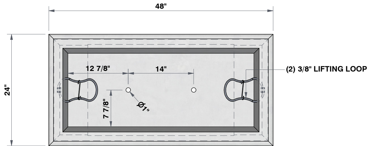
TOP VIEW 1"=1'
