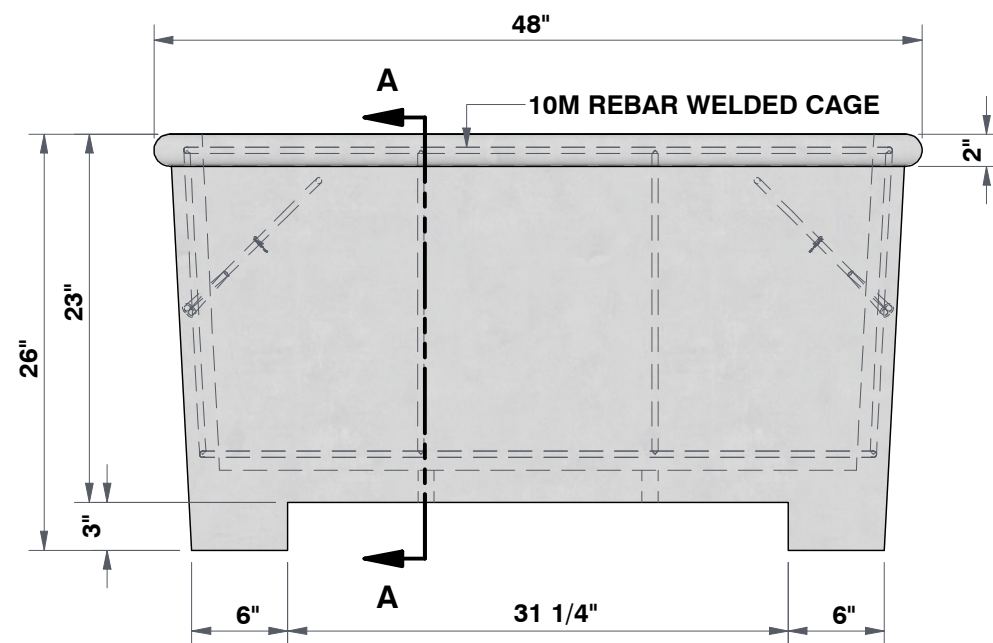
FRONT VIEW 1"=1'
