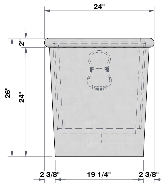
RIGHT SIDE VIEW 1"=1'
