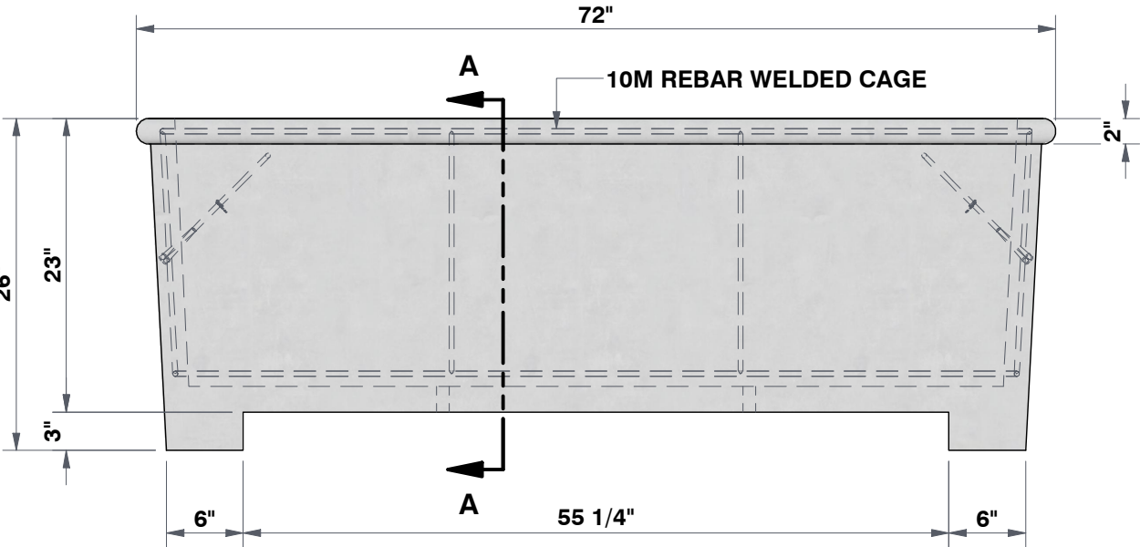
FRONT VIEW 7/8"=1'
