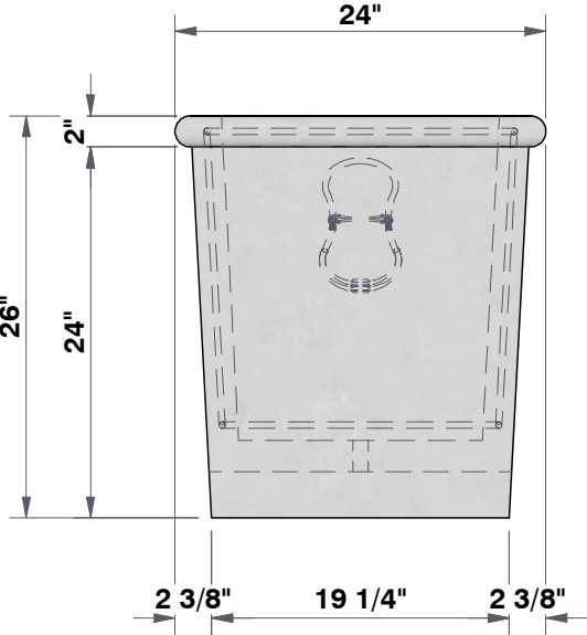
RIGHT SIDE VIEW 7/8"=1'
