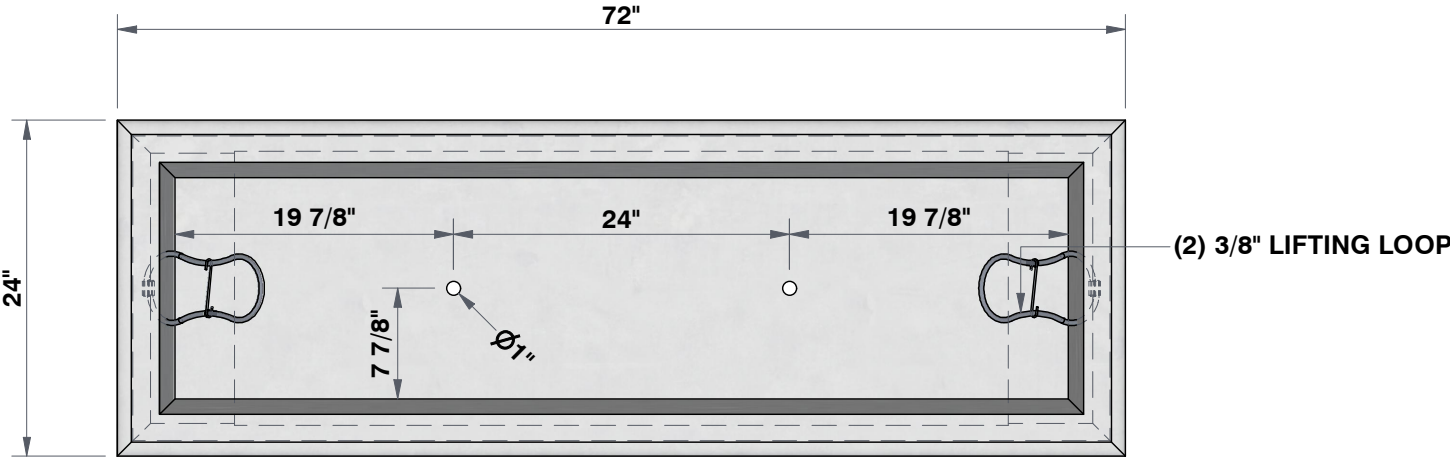
TOP VIEW 7/8"=1'
