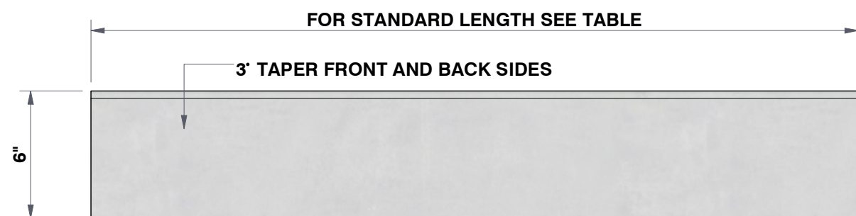
FRONT VIEW 1 7/8" = 1'
