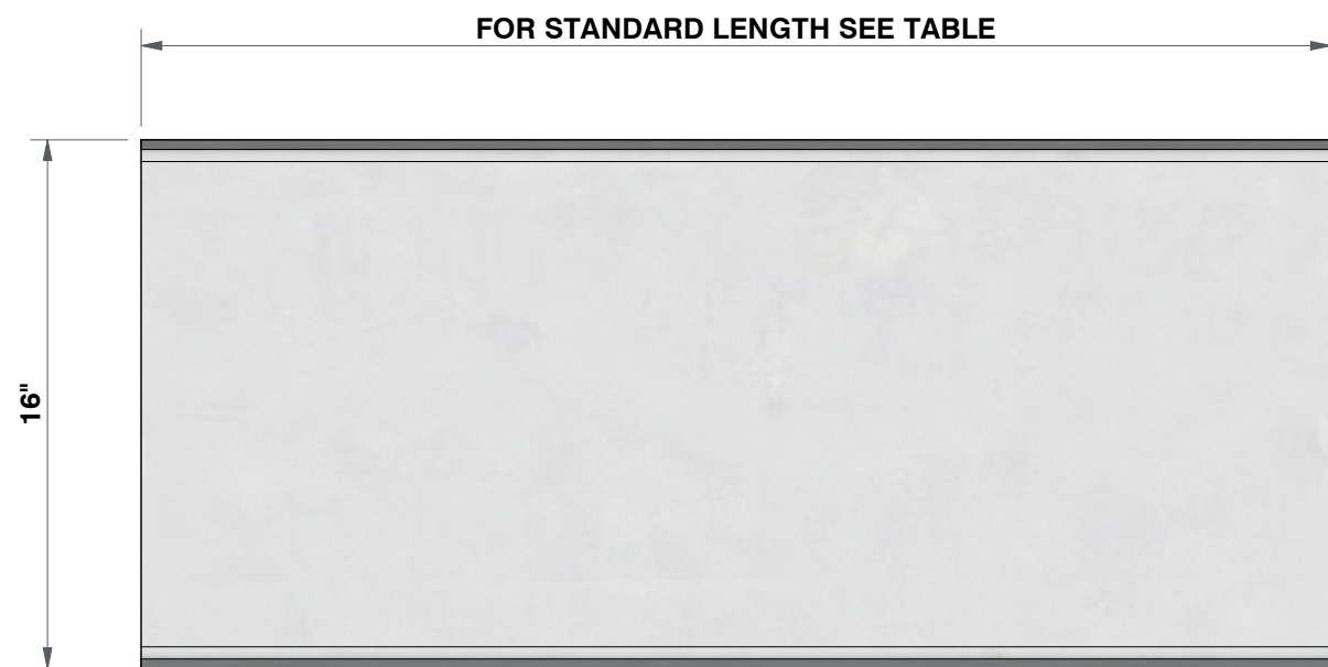
TOP VIEW 1 7/8" = 1'
