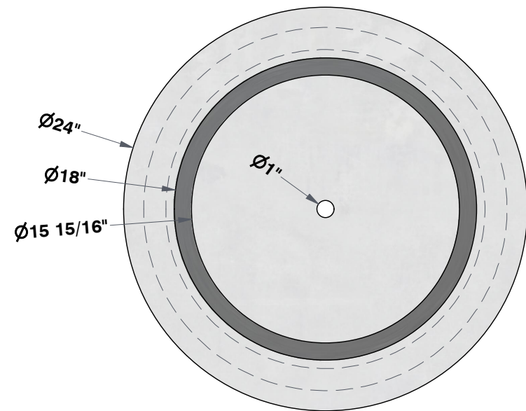
TOP VIEW 1 1/2"=1'
