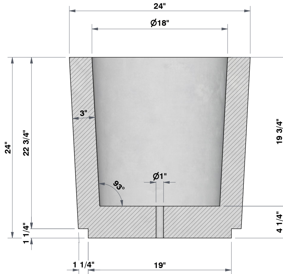
SECTION A-A 1 1/2"=1'
