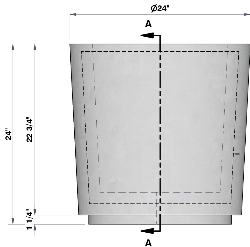
FRONT VIEW 1 1/2"=1'
