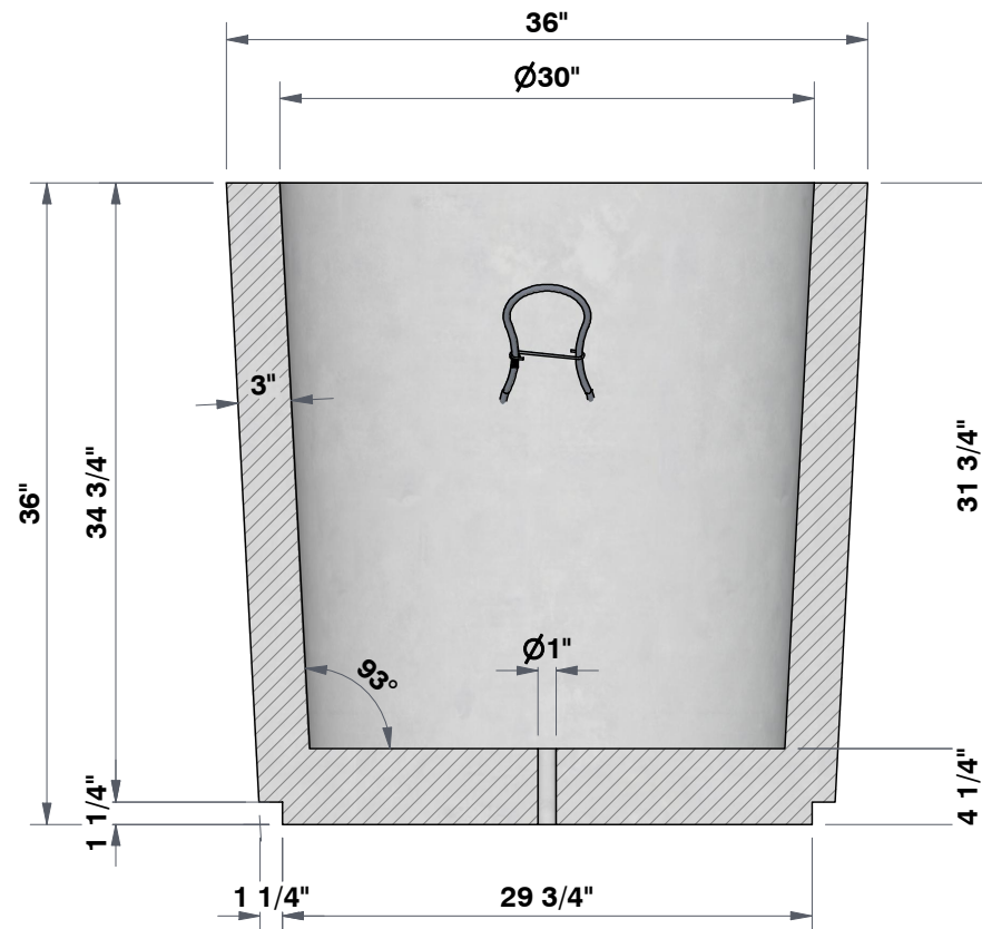
SECTION A-A 1"=1'
