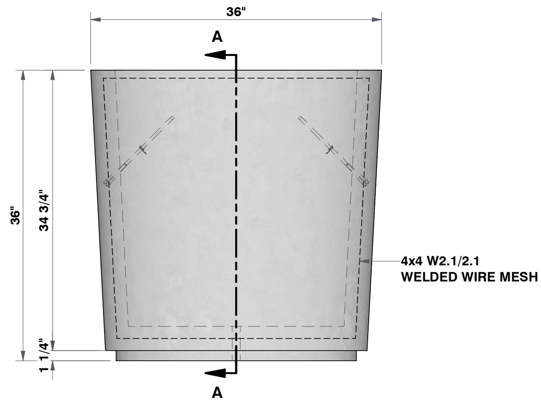
FRONT VIEW 1"=1'
