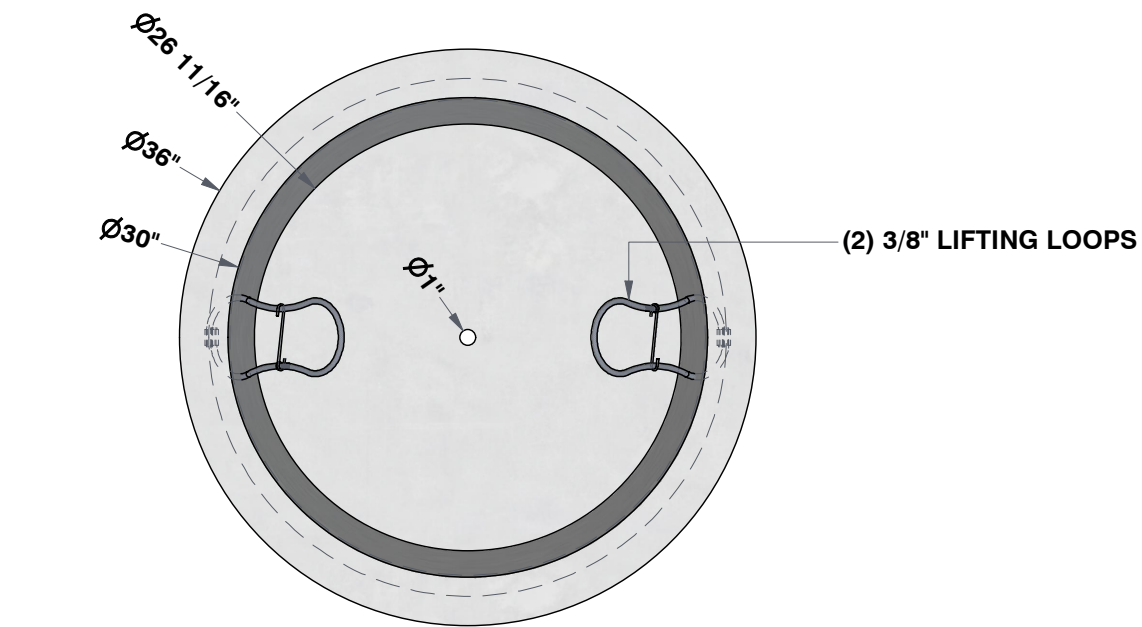
TOP VIEW 1"=1'
