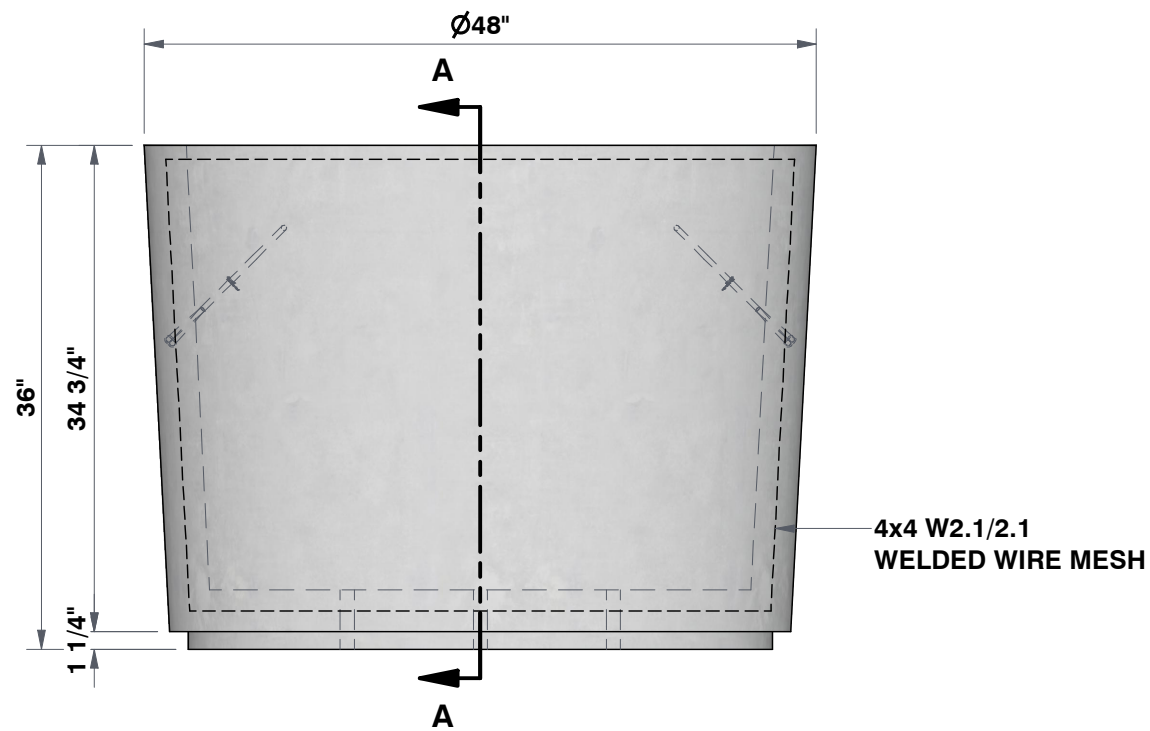
FRONT VIEW 7/8"=1'
