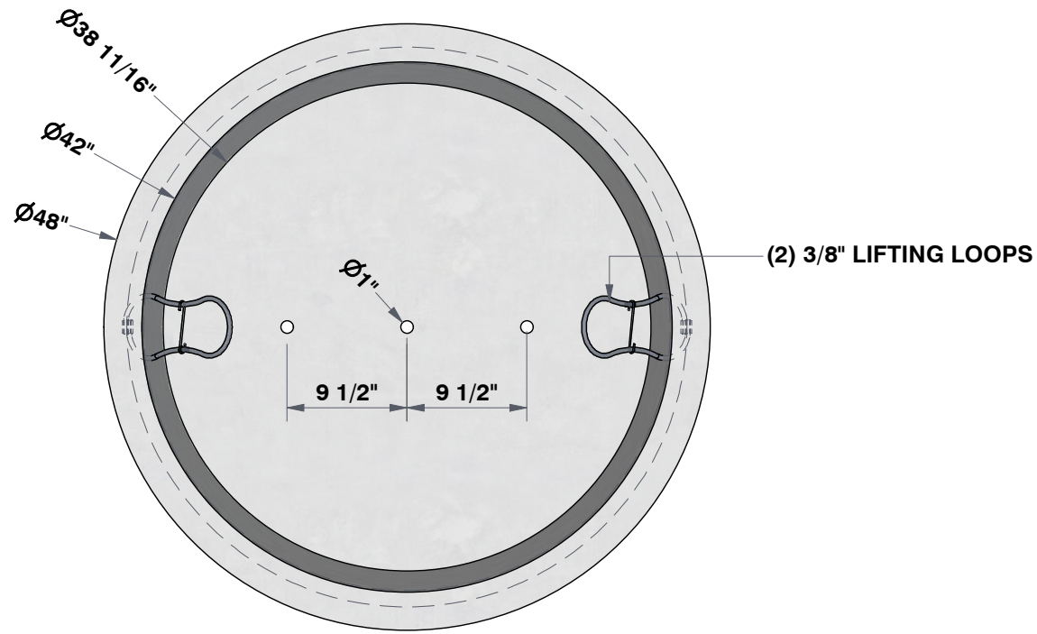
TOP VIEW 7/8"=1'
