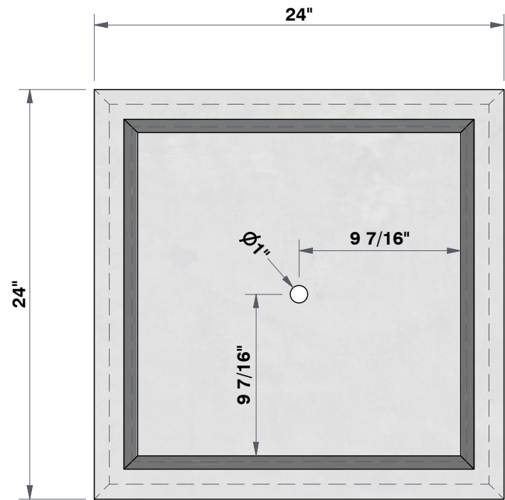
TOP VIEW 1 1/2"=1'
