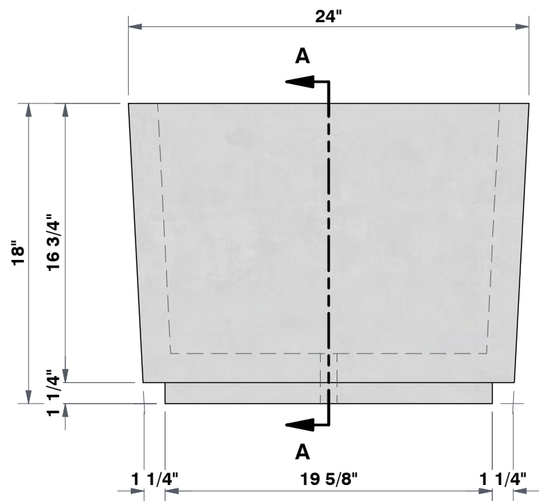
FRONT VIEW 1 1/2"=1'
