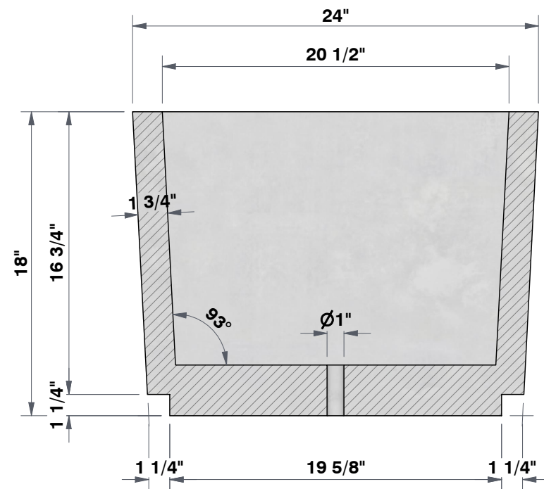
SECTION A-A 1 1/2"=1'
