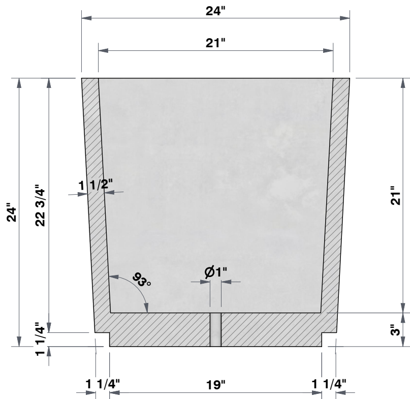
SECTION A-A 1 3/8"=1'
