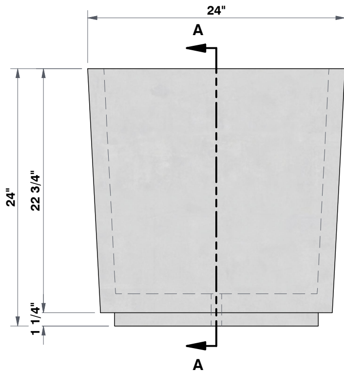
FRONT VIEW 1 3/8"=1'
