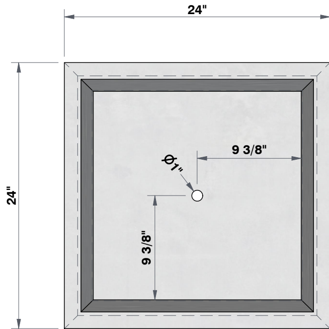
TOP VIEW 1 3/8"=1'
