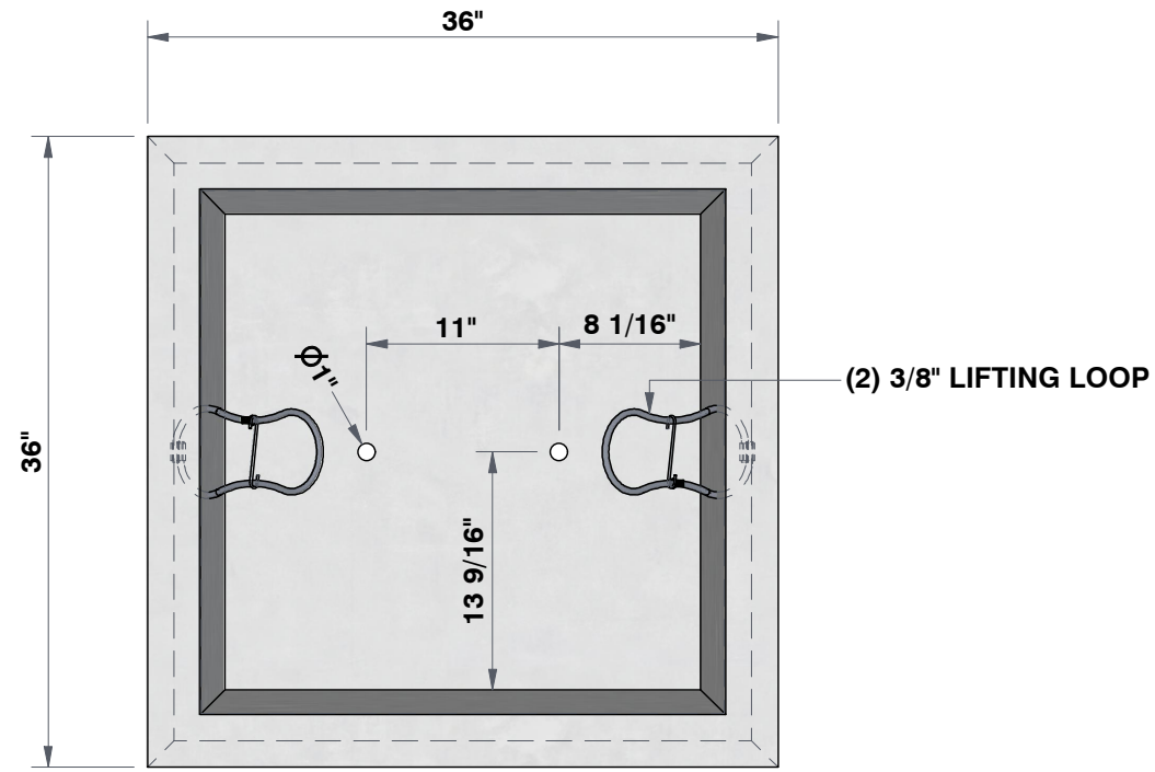
TOP VIEW 1"=1'
