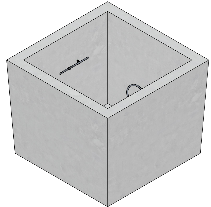
ISOMETRIC VIEW 1"=1'
