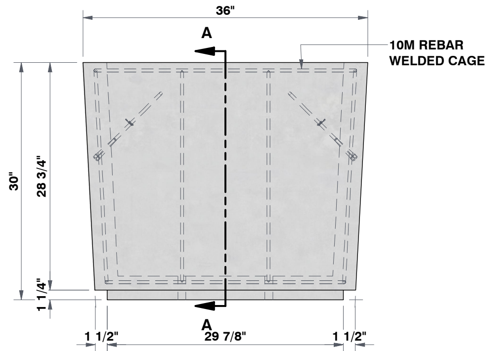
FRONT VIEW 1"=1'
