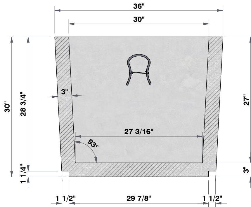
SECTION A-A 1"=1'
