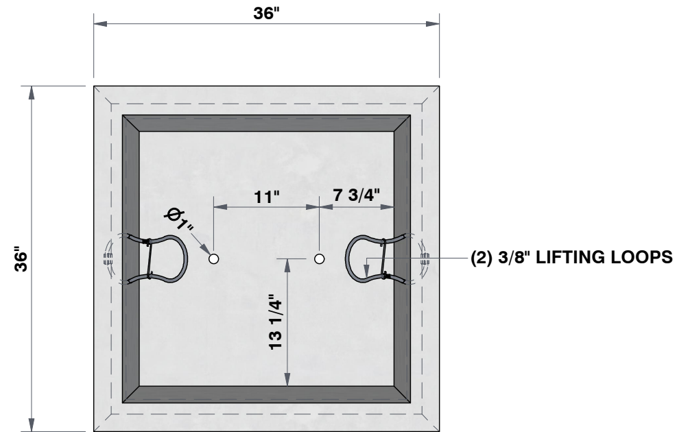
TOP VIEW 7/8"=1'
