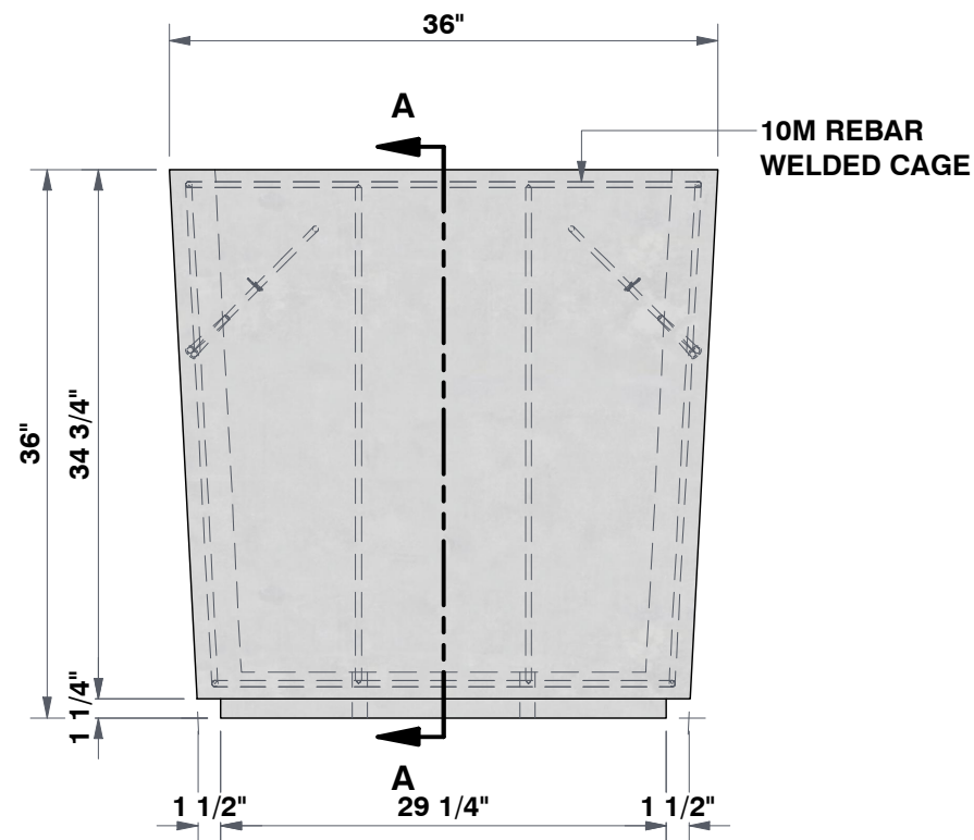
FRONT VIEW 7/8"=1'
