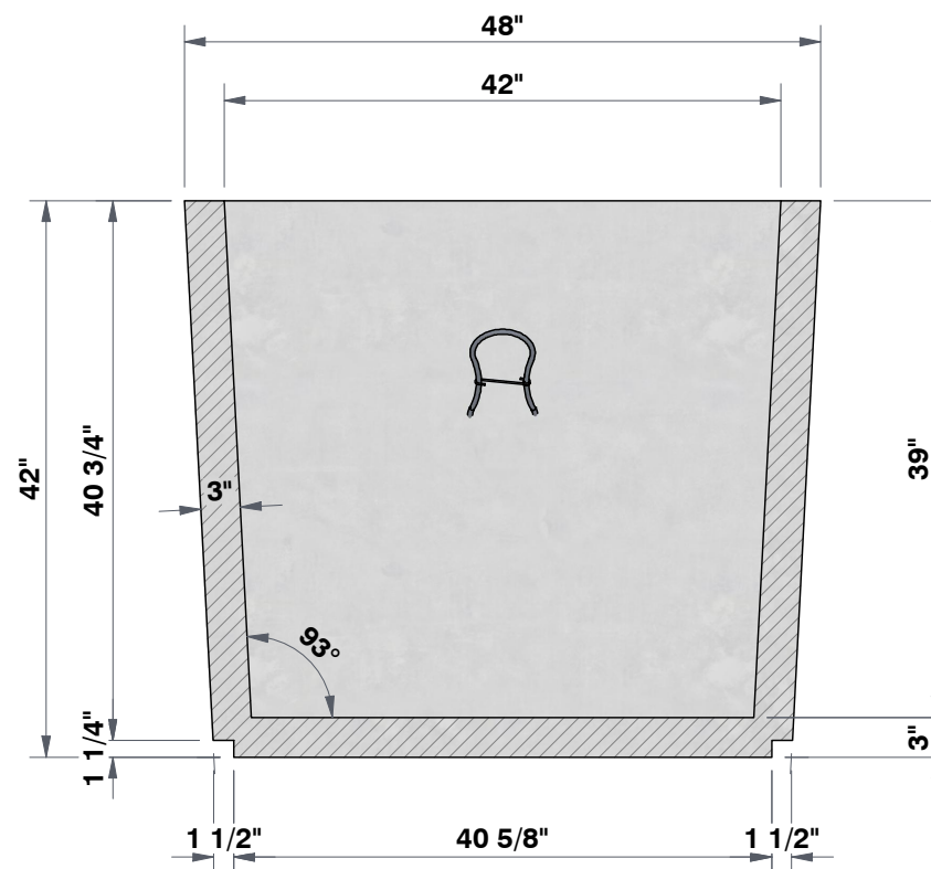
SECTION A-A 3/4" = 1'
