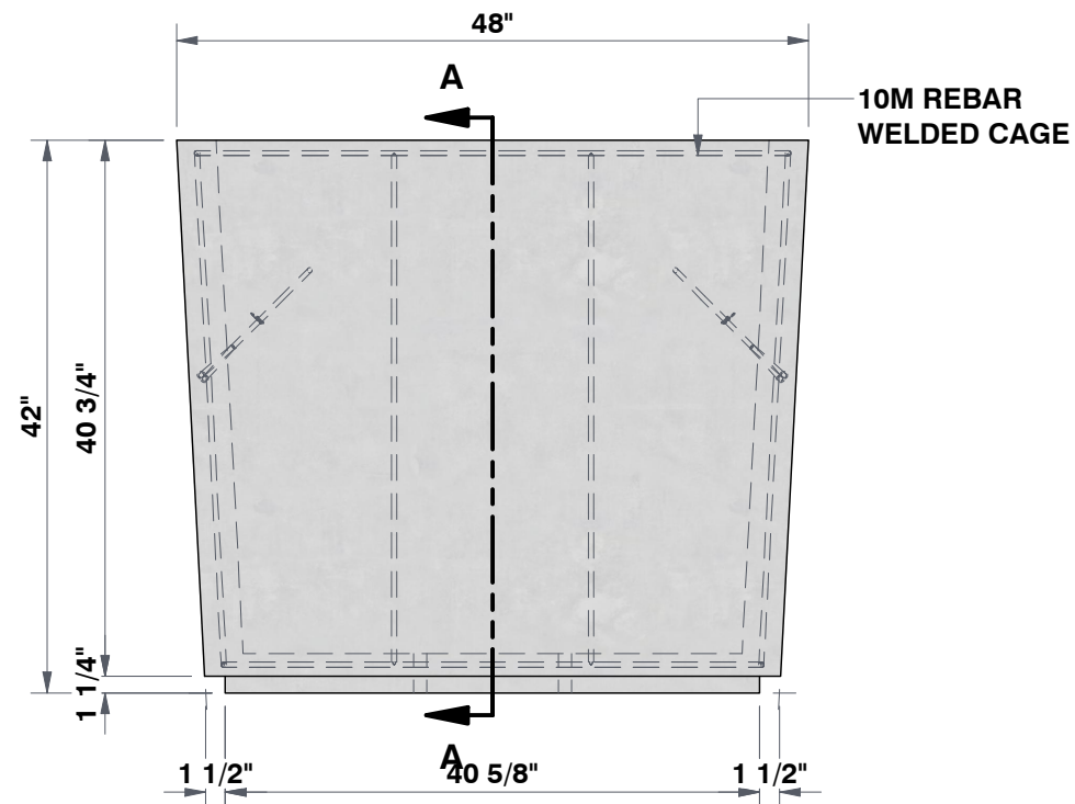
FRONT VIEW 3/4" = 1'
