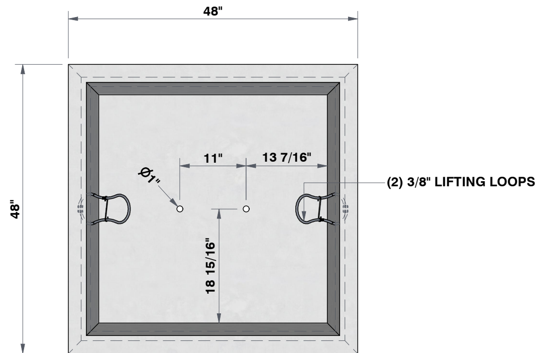
TOP VIEW 3/4" = 1'
