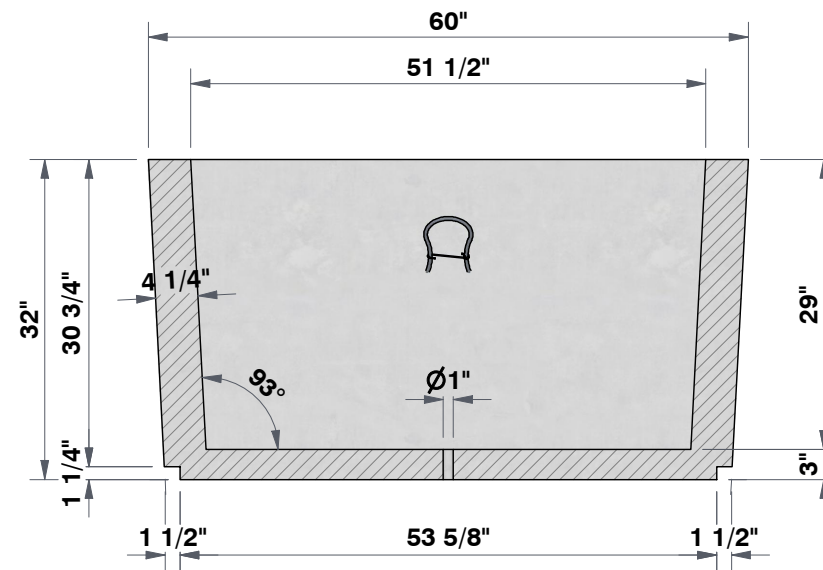
SECTION A-A 5/8"=1'
