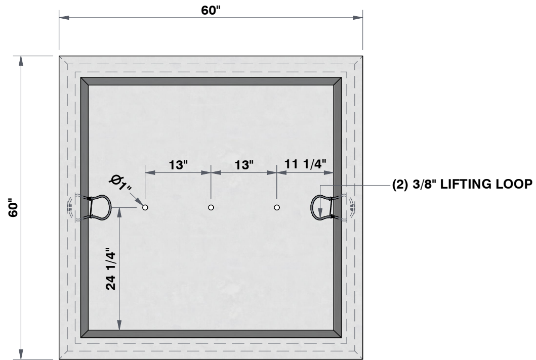
TOP VIEW 5/8"=1'
