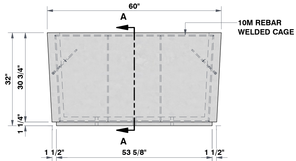
FRONT VIEW 5/8"=1'
